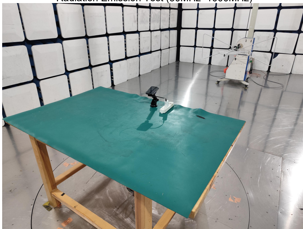
Radiation Emission Test (30MHz~1000MHz)
