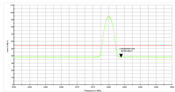
3DH5-Channel 78: Average
