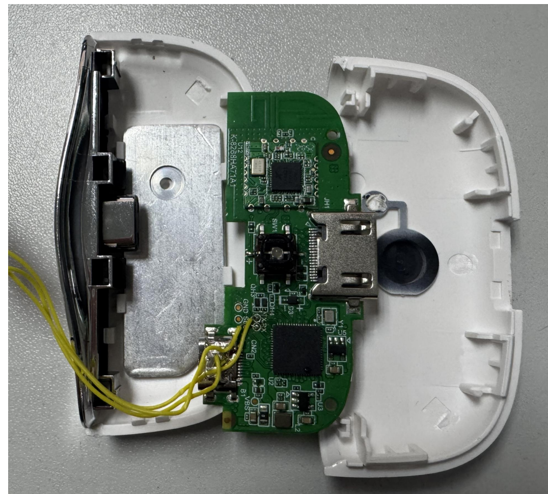
Receiver
