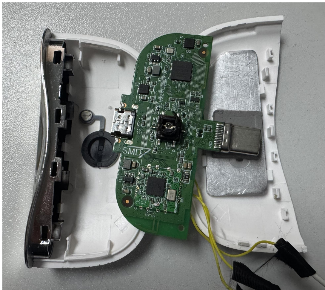
Transmitter
