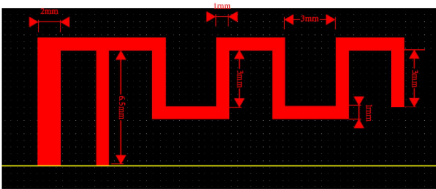
Antenna Layout & module on the system board
