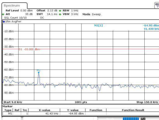
Band5_10MHz_QPSK_20525_1RB#0_0.009~0.15
