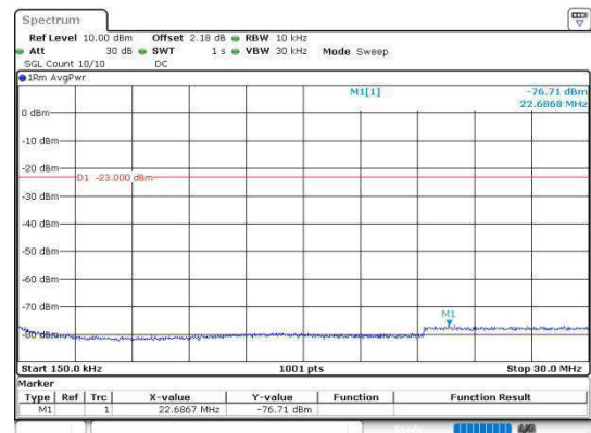
Band5_5MHz_QPSK_20525_1RB#0_0.15~30
