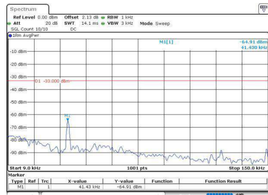
Band5_1.4MHz_64QAM_20525_1RB#0_0.009~0.15
