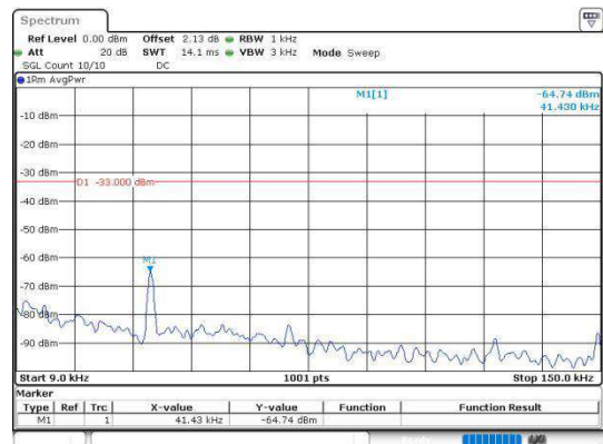
Band5_5MHz_64QAM_20525_1RB#0_0.009~0.15
