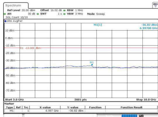
Band5_10MHz_16QAM_20600_1RB#0_3000~10000
