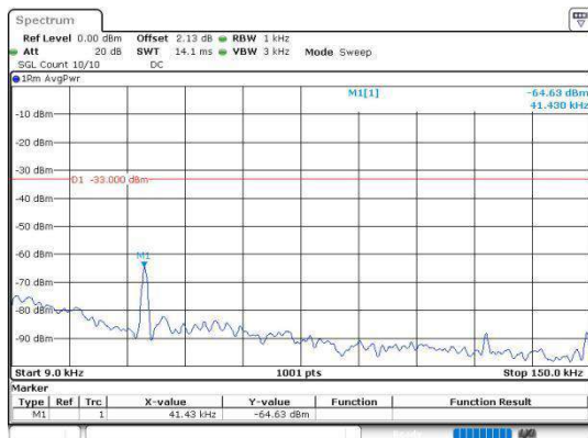
Band5_5MHz_64QAM_20625_1RB#0_0.009~0.15
