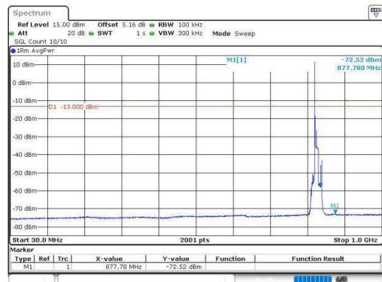
Band5_10MHz_64QAM_20450_1RB#0_30~1000
