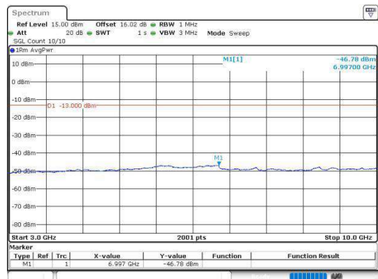
Band5_10MHz_64QAM_20600_1RB#0_3000~10000
