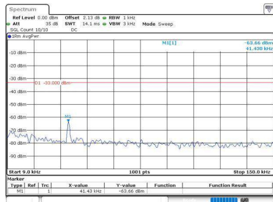
Band5_10MHz_16QAM_20450_1RB#0_0.009~0.15
