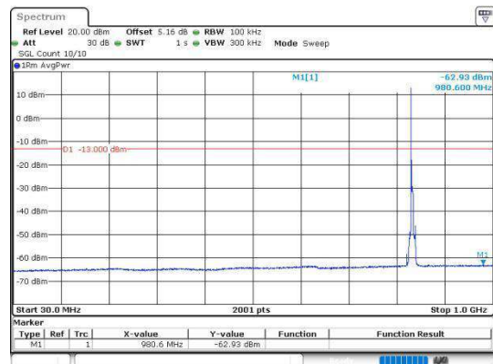
Band5_5MHz_16QAM_20525_1RB#0_30~1000
