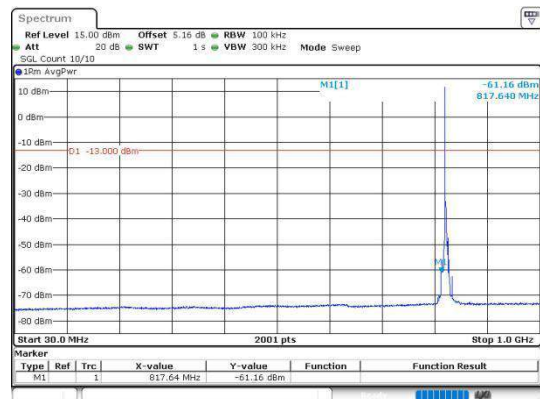
Band5_3MHz_64QAM_20415_1RB#0_30~1000
