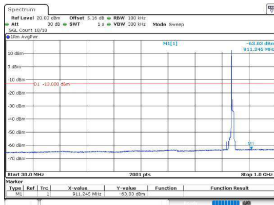
Band5_10MHz_QPSK_20600_1RB#0_30~1000
