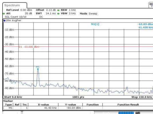
Band5_1.4MHz_64QAM_20643_1RB#0_0.009~0.15
