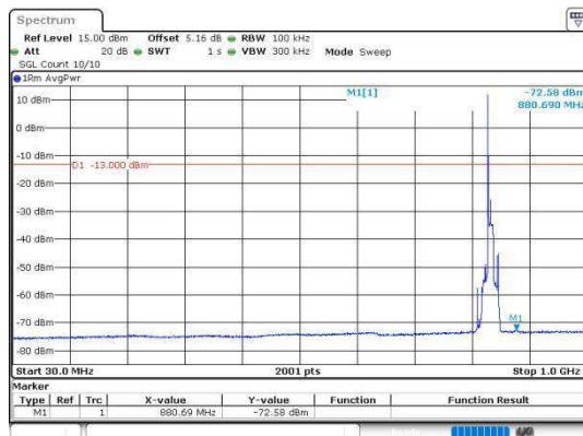
Band5_10MHz_64QAM_20525_1RB#0_30~1000
