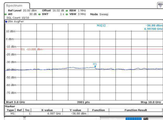
Band5_5MHz_16QAM_20625_1RB#0_3000~10000
