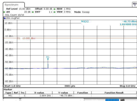
Band5_10MHz_64QAM_20525_1RB#0_1000~3000
