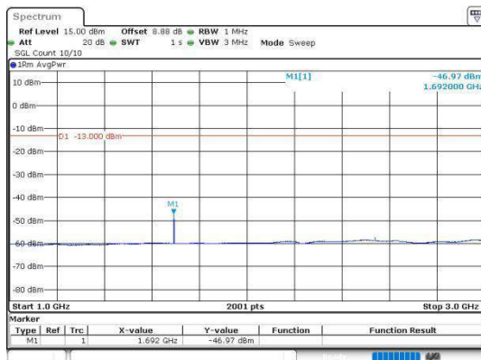
Band5_3MHz_64QAM_20635_1RB#0_1000~3000
