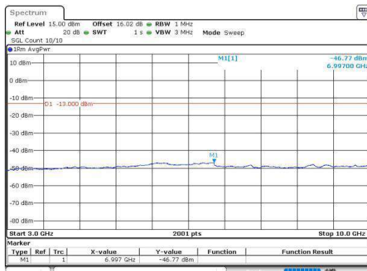
Band5_1.4MHz_64QAM_20407_1RB#0_3000~10000
