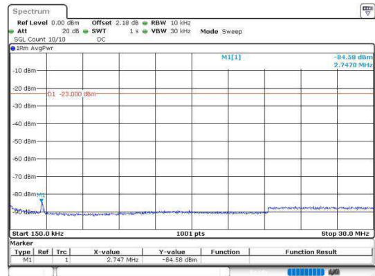
Band5_5MHz_64QAM_20425_1RB#0_1000~3000
