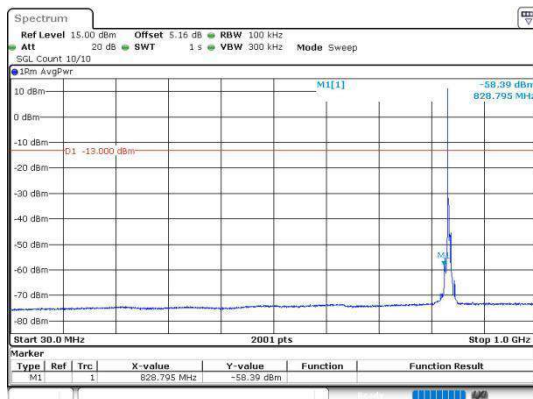
Band5_3MHz_64QAM_20525_1RB#0_30~1000
