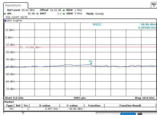
Band5_3MHz_16QAM_20635_1RB#0_3000~10000
