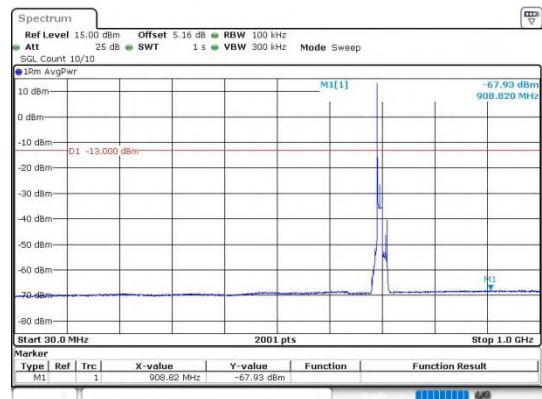
Band12_10MHz_64QAM_23060_1RB#0_30~1000
