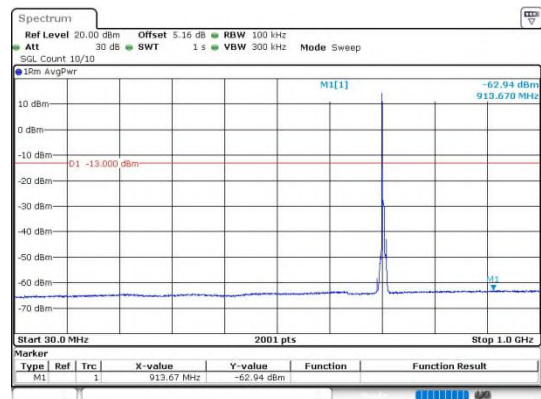
Band17_5MHz_16QAM_23790_1RB#0_30~1000
