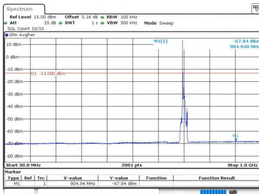
Band12_10MHz_64QAM_23095_1RB#0_30~1000
