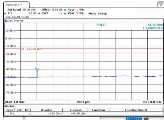
Band17_10MHz_QPSK_23800_1RB#0_1000~3000
