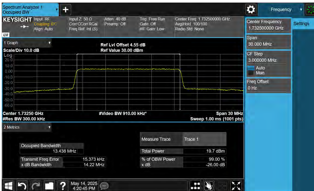
B4\Band4-15MHz-64QAM-20175-75RB#0
