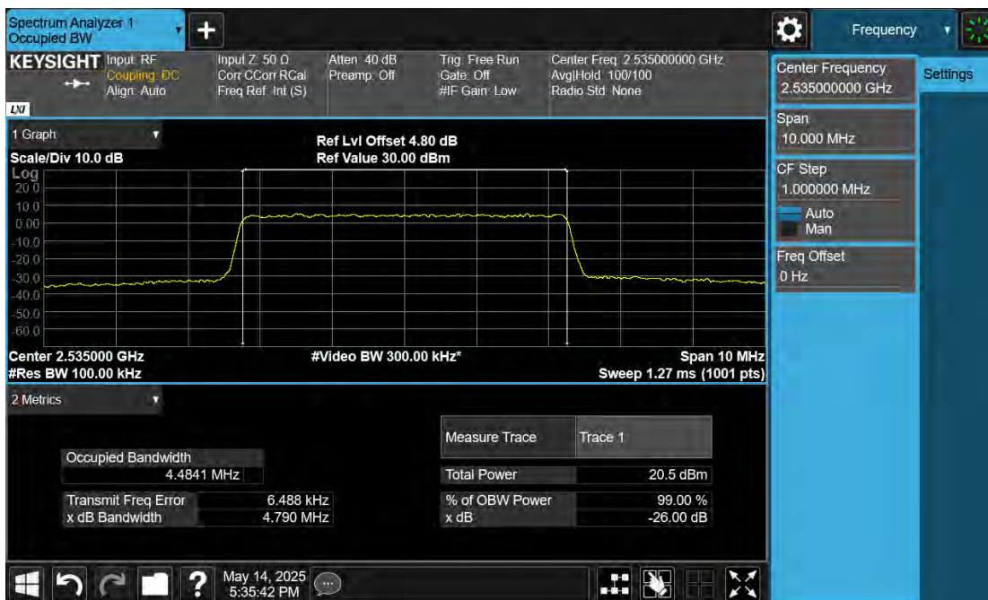
B7\Band7-5MHz-16QAM-21100-25RB#0
