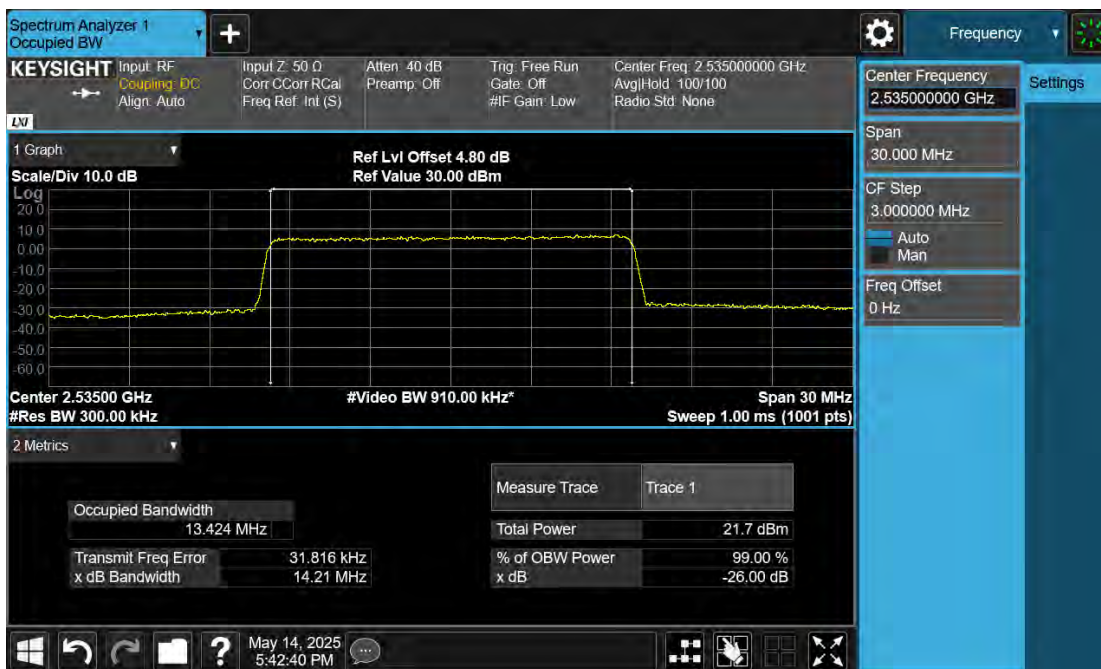
B7\Band7-15MHz-QPSK-21100-75RB#0
