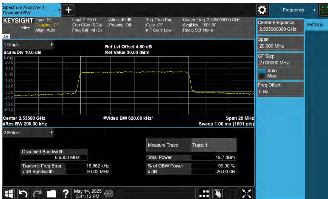
B7\Band7-10MHz-64QAM-21100-50RB#0
