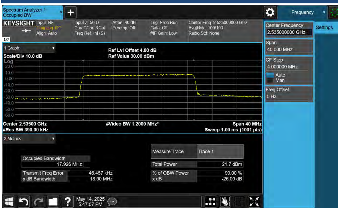
B7\Band7-20MHz-QPSK-21100-100RB#0
