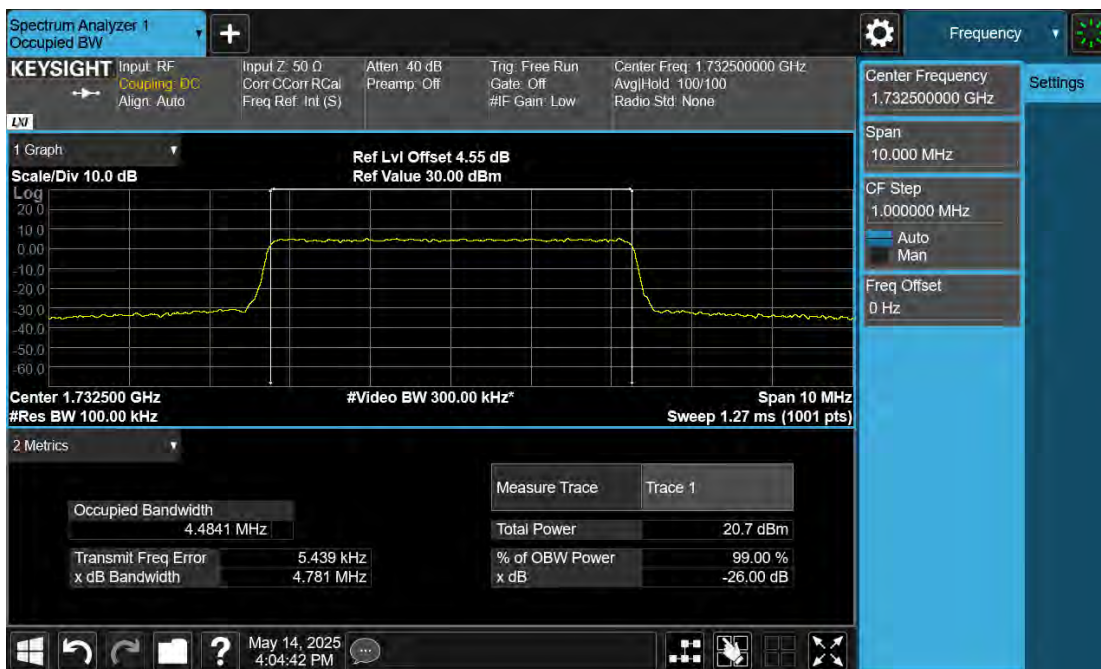
B4\Band4-5MHz-16QAM-20175-25RB#0
