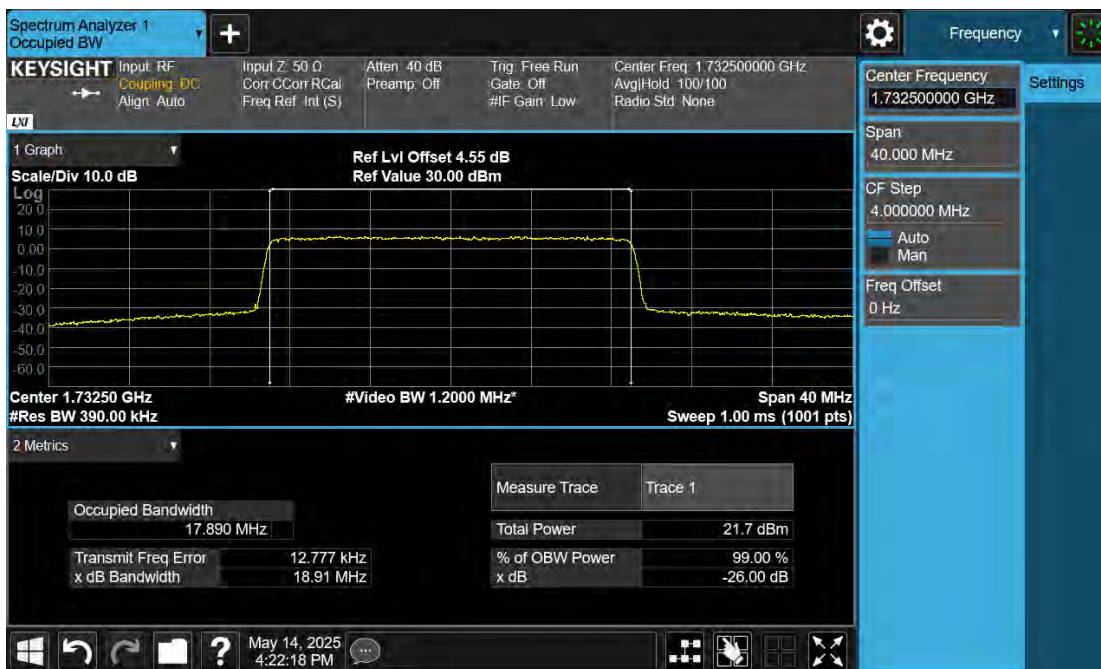
B4\Band4-20MHz-QPSK-20175-100RB#0
