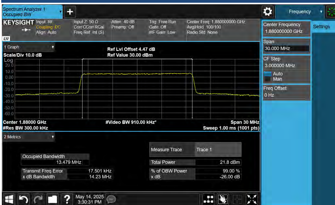
B2\Band2-15MHz-QPSK-18900-75RB#0
