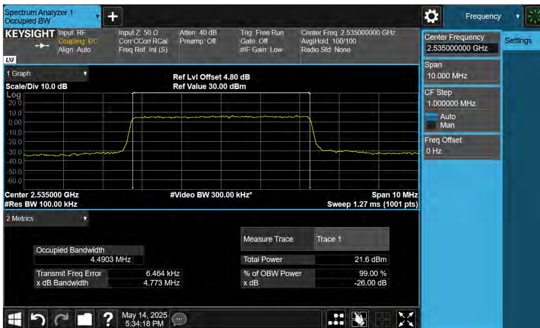
B7\Band7-5MHz-QPSK-21100-25RB#0
