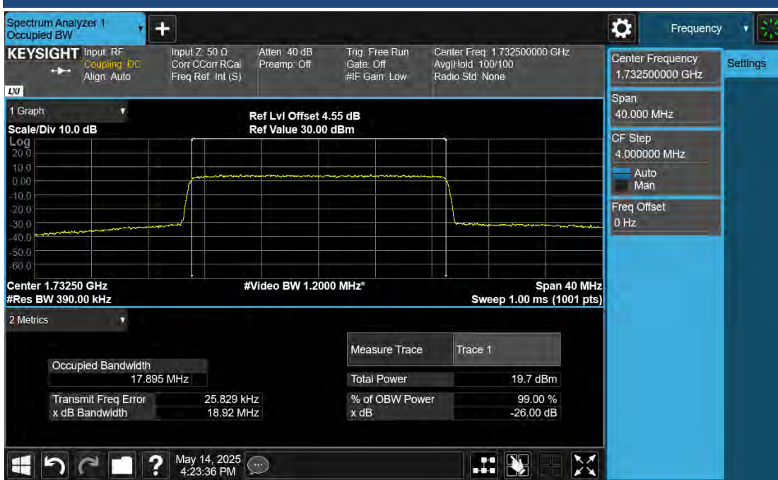
B4\Band4-20MHz-64QAM-20175-100RB#0
