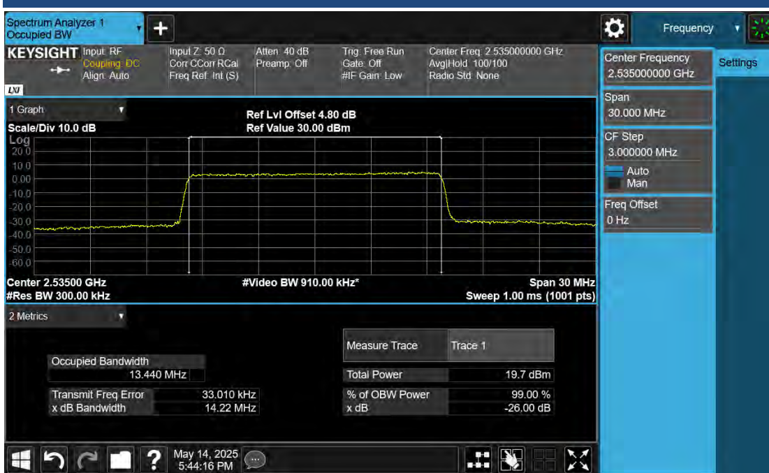
B7\Band7-15MHz-64QAM-21100-75RB#0
