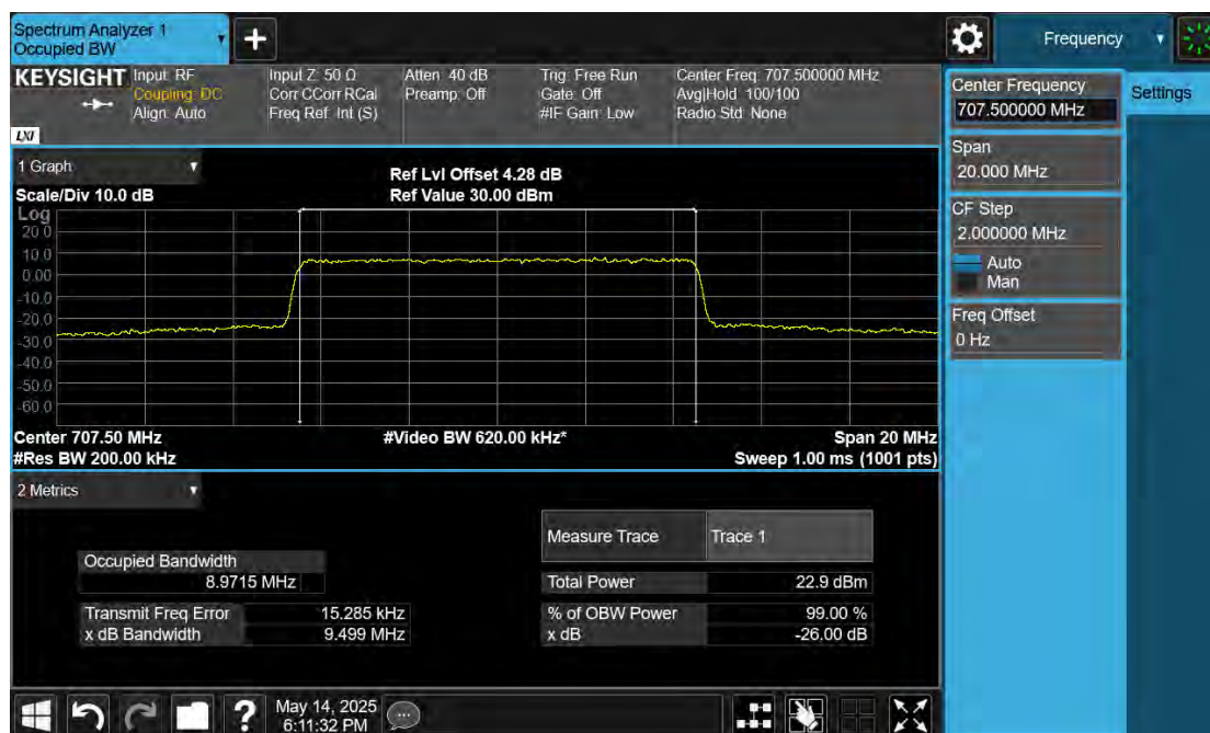
B12\Band12-10MHz-QPSK-23095-50RB#0
