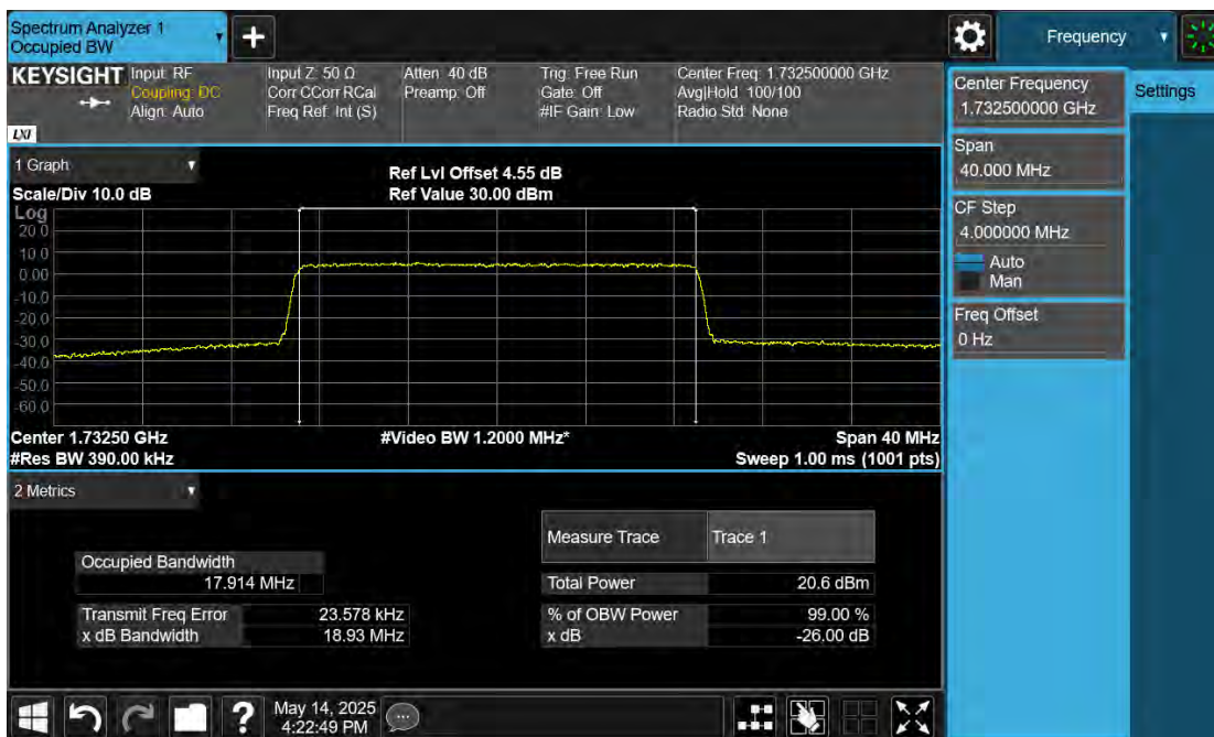
B4\Band4-20MHz-16QAM-20175-100RB#0
