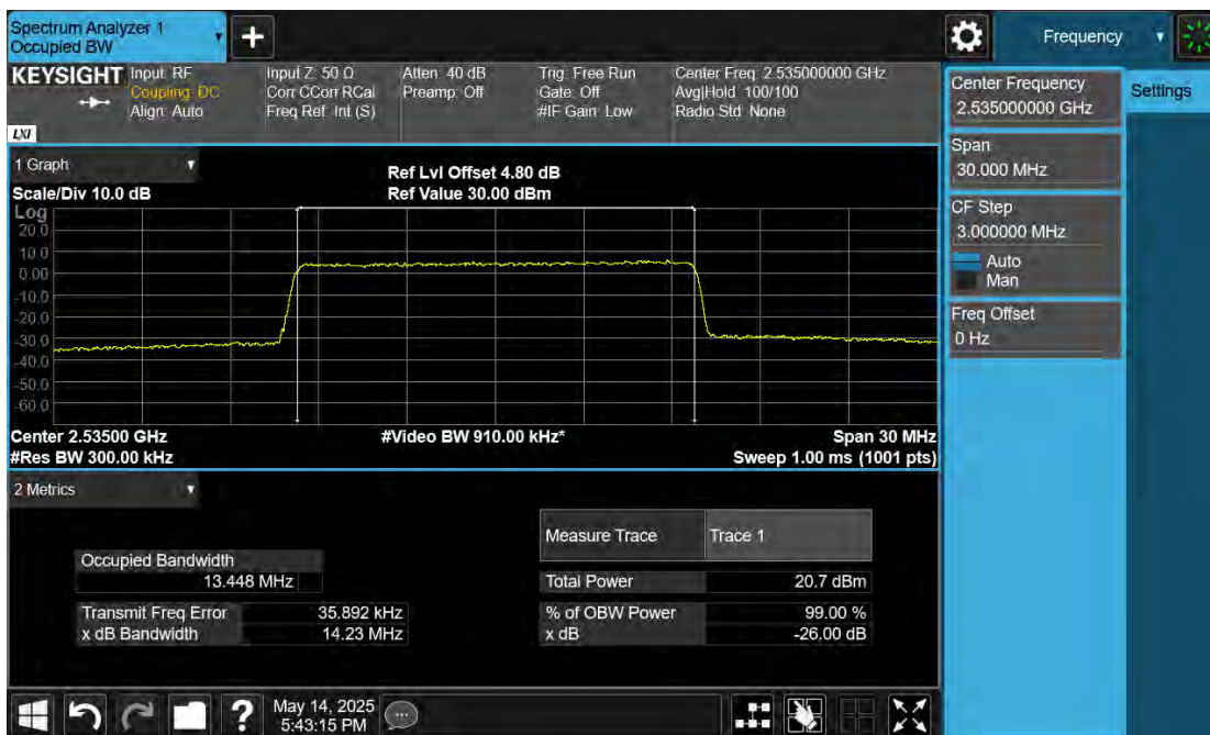
B7\Band7-15MHz-16QAM-21100-75RB#0
