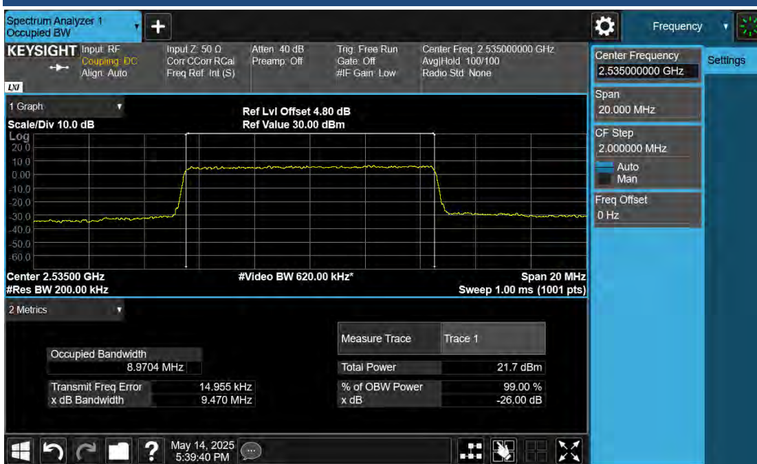
B7\Band7-10MHz-QPSK-21100-50RB#0
