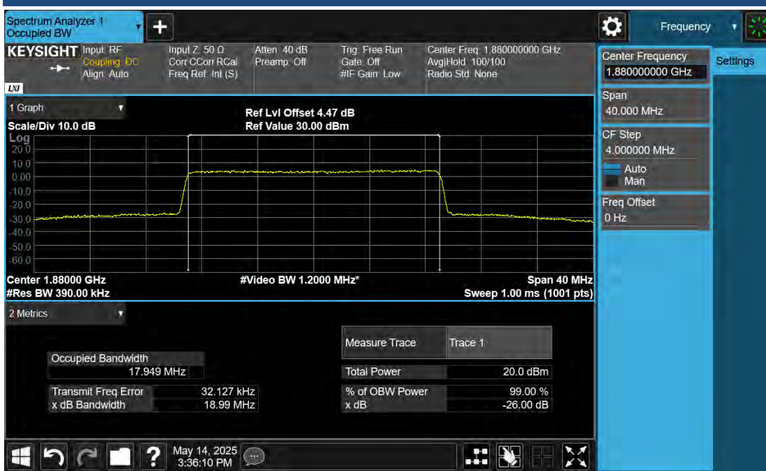
B2\Band2-20MHz-64QAM-18900-100RB#0
