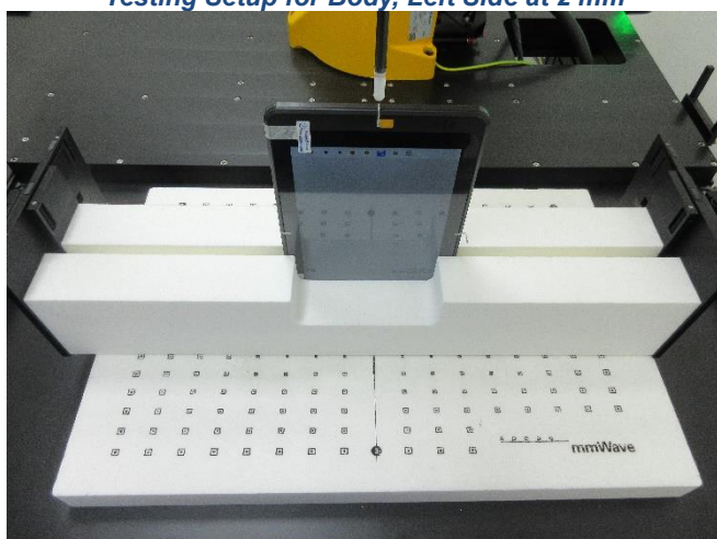
Testing Setup for Body, Left Side at 2 mm
