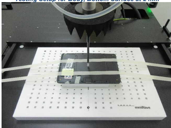
Testing Setup for Body, Bottom Surface at 2 mm
