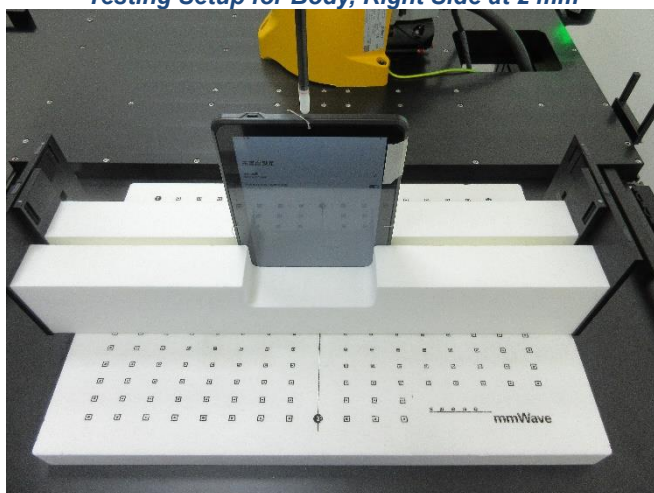
Testing Setup for Body, Right Side at 2 mm
