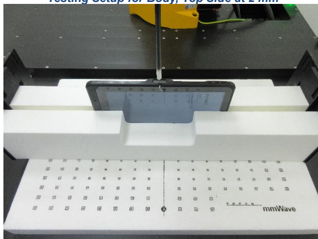
Testing Setup for Body, Top Side at 2 mm
