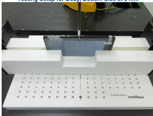
Testing Setup for Body, Bottom Side at 2 mm
