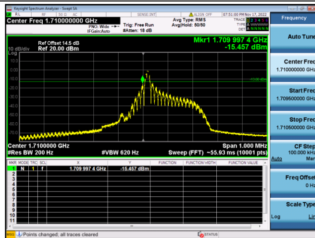
BPSK Low channel-1@0
