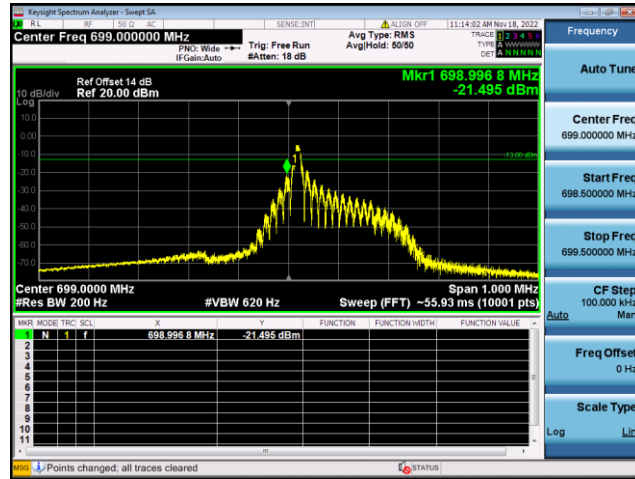
QPSK Low channel-12@0
