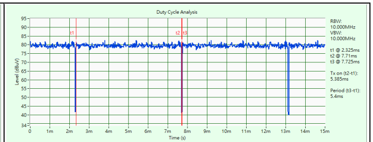
802.11g
