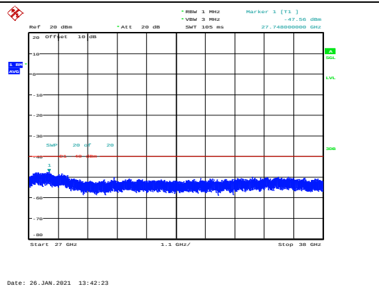
B48-10-20-CSE-H-Q64-2
