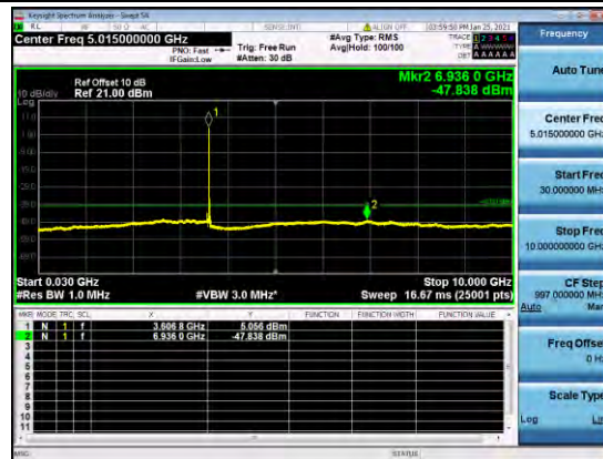
B48-20-10-CSE-M-QPSK-3
