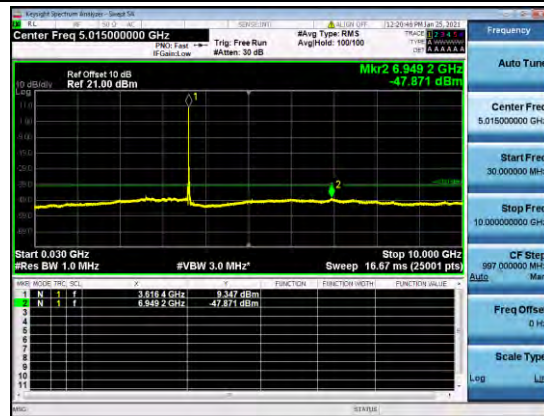
B48-10-20-CSE-M-Q64-3
