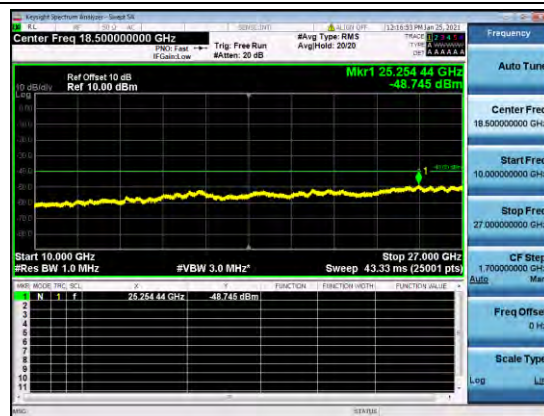
B48-10-20-CSE-M-Q64-1
