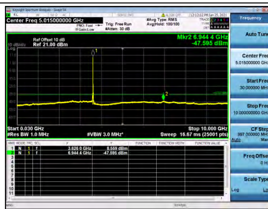
B48-10-20-CSE-M-QPSK-3
