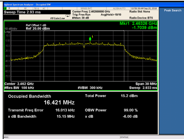
11g-HCH
