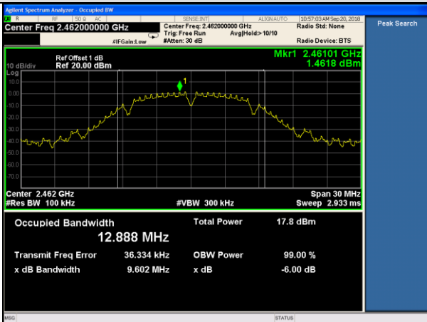
11b-HCH
