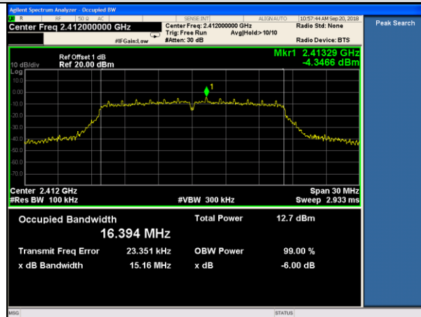
11g-LCH
