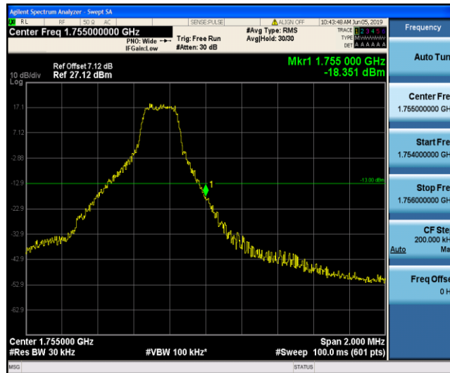
Band4_1.4MHz_16QAM_20393_1RB#5
