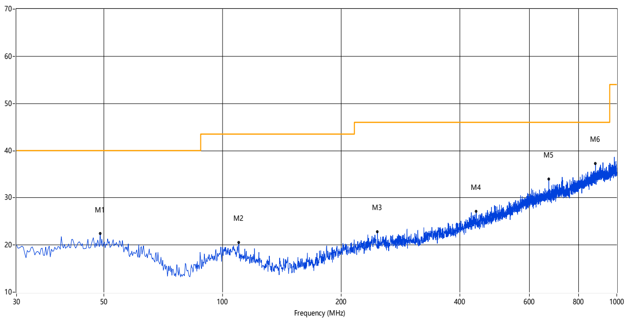
30 MHz to 1 GHz, ANT V (TX2402)
