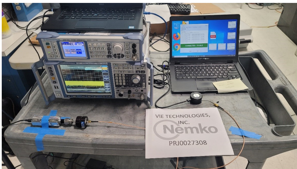
Figure 6 – Test setup: power meter, antenna conducted port.
