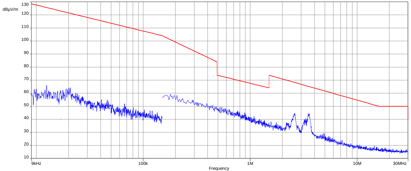
Plot No. 7: Tx magnetic, 9 kHz – 30 MHz
