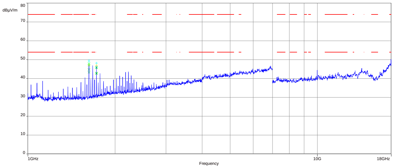
Plot No. 8: 1 GHz to 18 GHz
