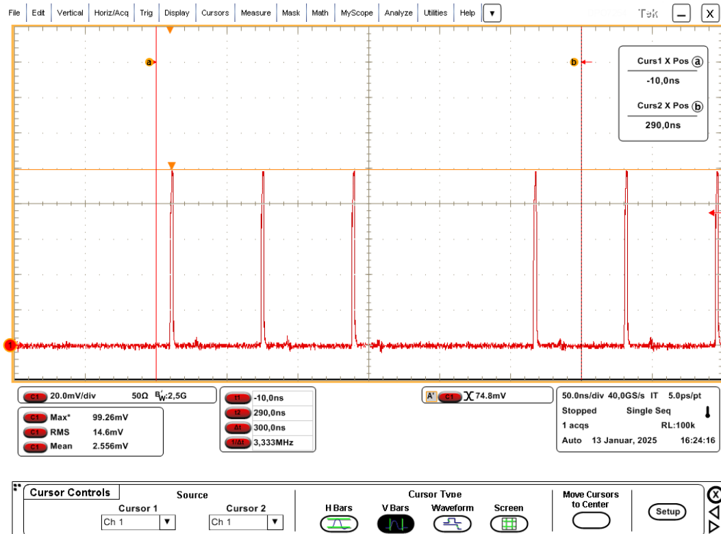
Plot 2: EUT emission, V_{\max,EUT} , V_{\text{avg}0.3\mu\text{s},EUT}
