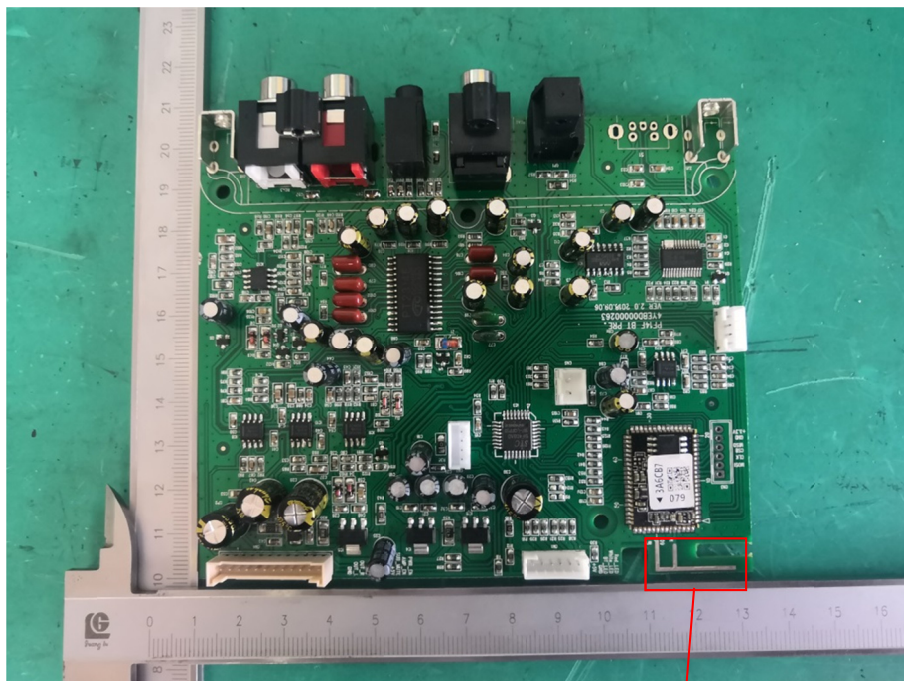
Bluetooth Antenna
