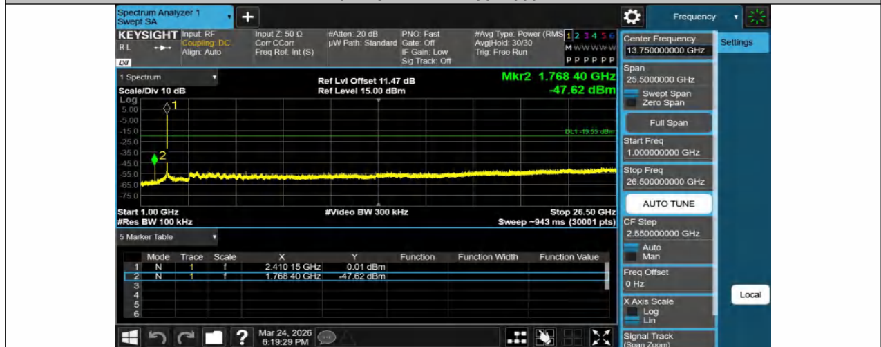
11N20SISO-Ant1-2412-1000~26500-PASS
