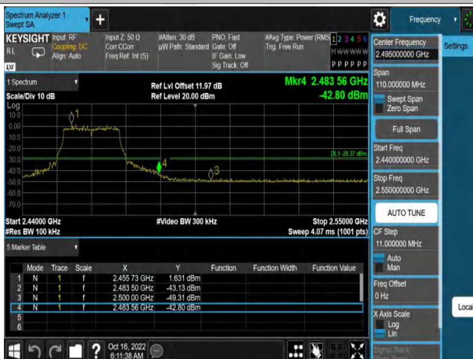
11N20SISO_Ant1_High_2462
