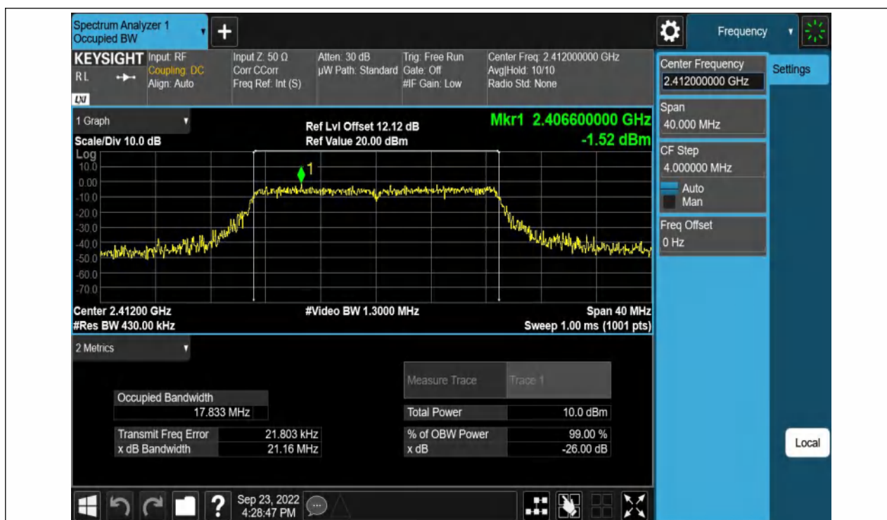
11N20SISO_Ant1_2412
