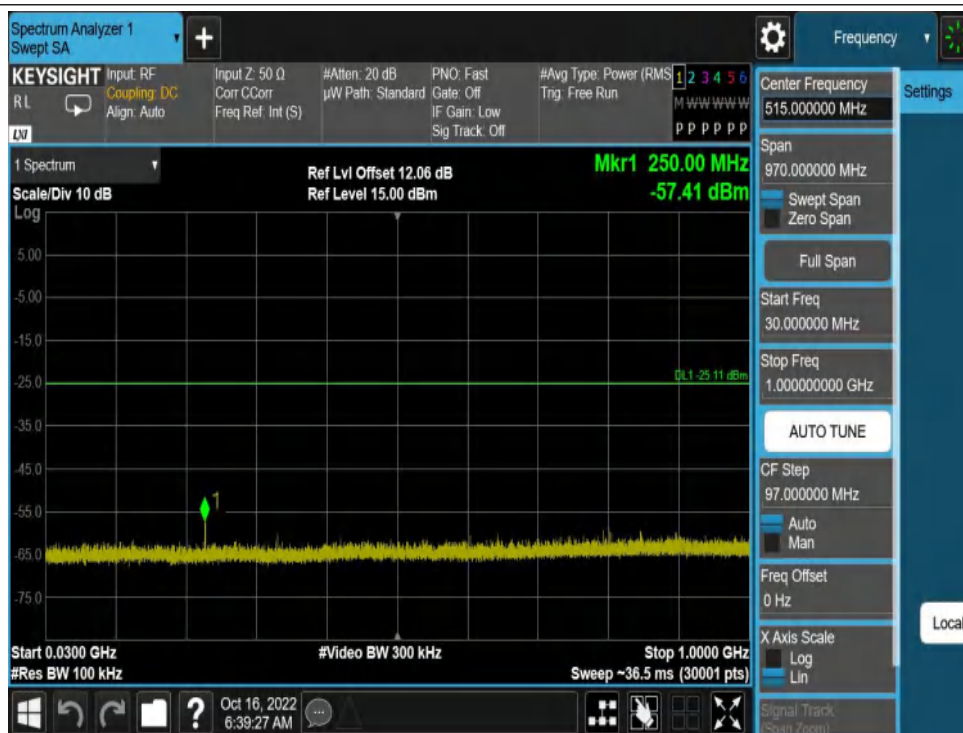
11B-Ant1-2437-30~1000
