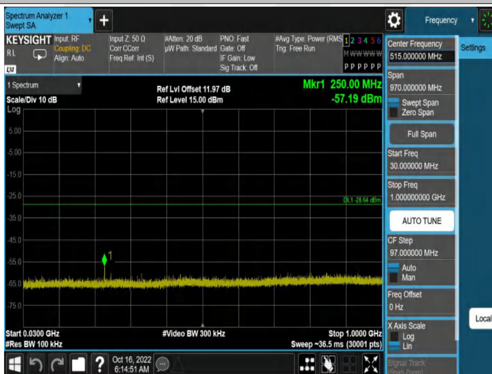
11N20SISO-Ant1-2462-30~1000
