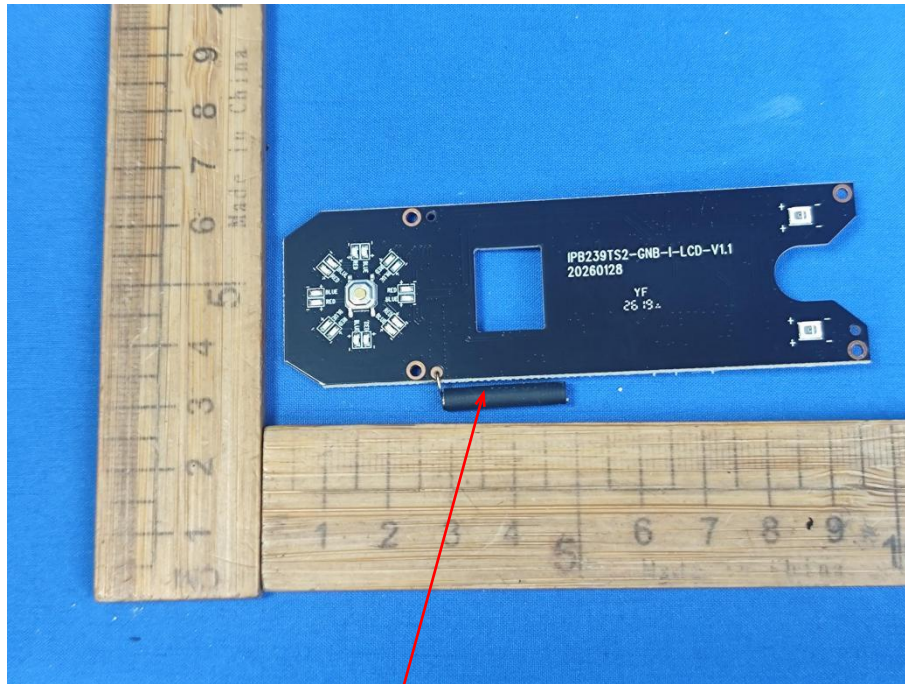
433MHz Antenna
