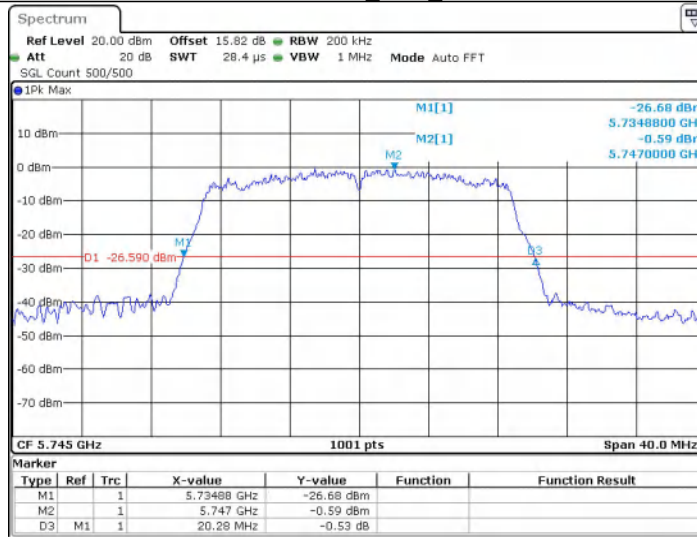
11AC20SISO_Ant1_5745
