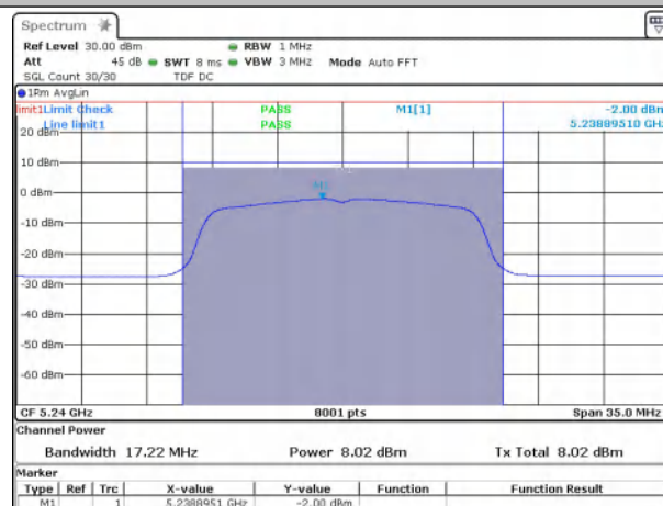
NTNV_802.11a(20M)_5240_54Mbps_ANT1
