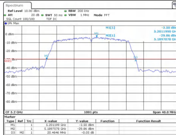
NTNV_802.11a(20M)_5200_54Mbps_ANT1
