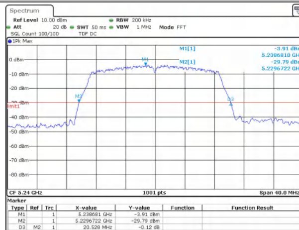
NTNV_802.11a(20M)_5240_54Mbps_ANT1
