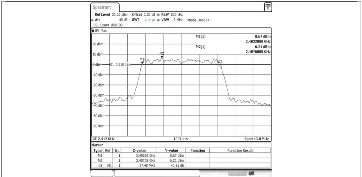
11N20SISO-Ant1-2412-PASS
