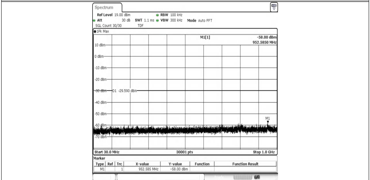
11N20SISO-Ant1-2412-0~Reference-PASS
