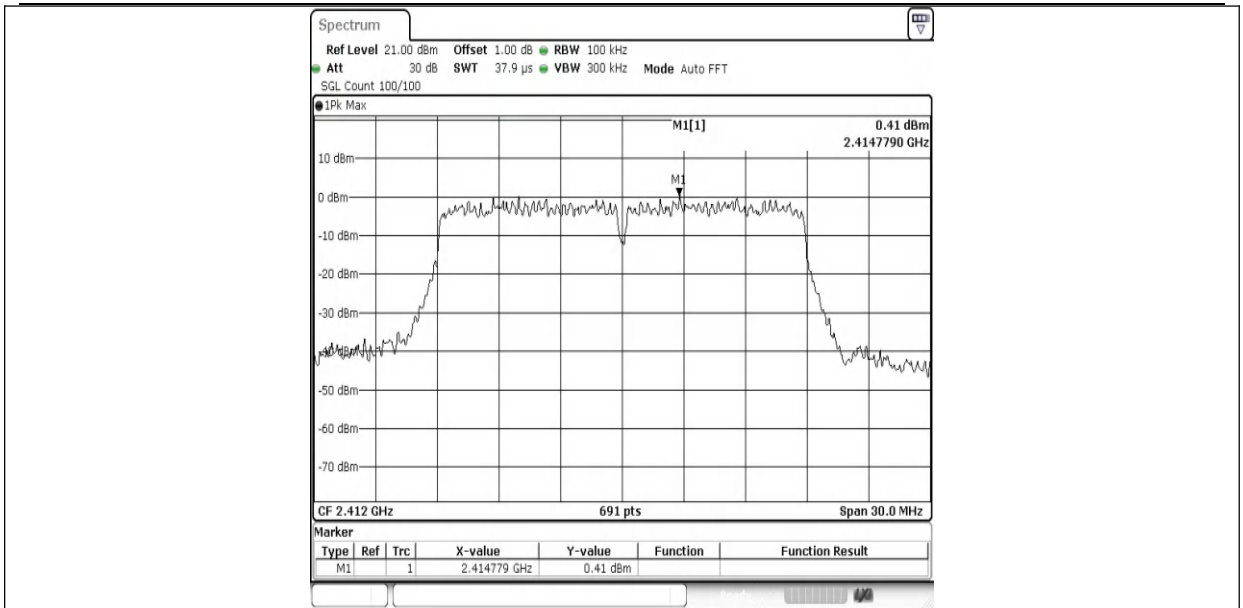
11N20SISO-Ant1-2412-0~Reference-PASS
