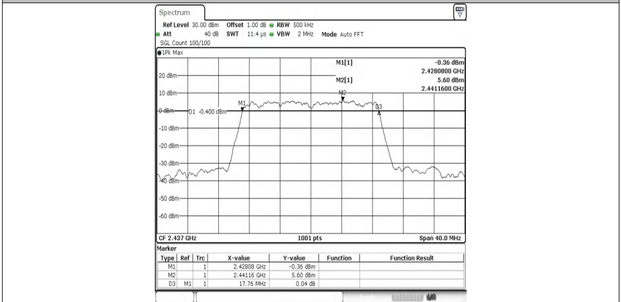
11N20SISO-Ant1-2437-PASS
