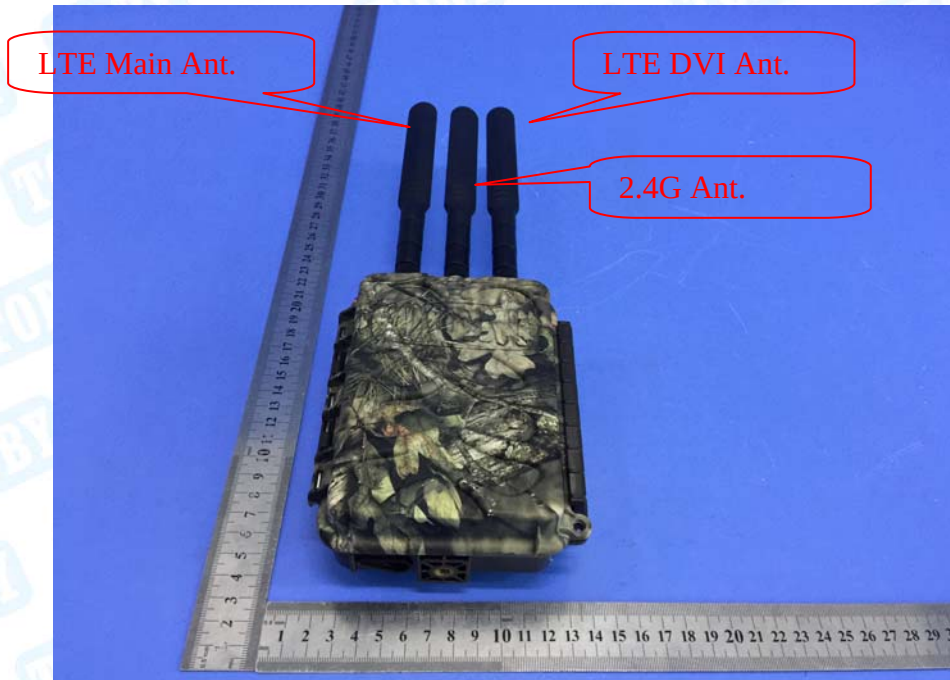
Photo 1 Appearance of EUT
