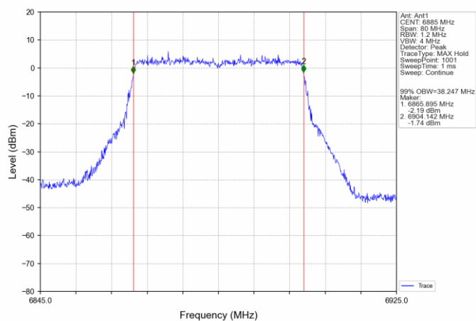
802.11ax(HEW40)_HCH_6885MHz_SU_ / Ant1_NTNV
