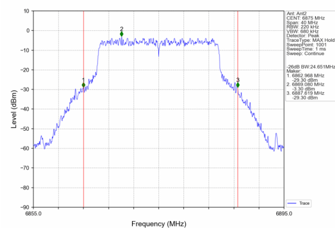
802.11ax(HEW20)_HCH_6875MHz_SU_ / Ant2_NTNV
