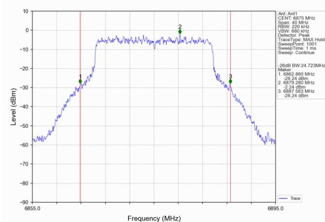
802.11ax(HEW20)_HCH_6875MHz_SU_ / Ant1_NTNV
