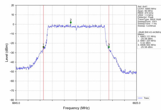
802.11ax(HEW40)_HCH_6885MHz_SU_ / Ant1_NTNV
