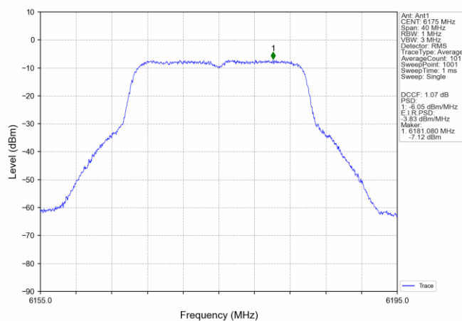
802.11ax(HEW20) MCH 6175MHz_SU / Ant1_NTNV
