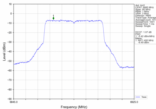
802.11ax(HEW40)_HCH_6885MHz_SU_ / Ant1_NTNV
