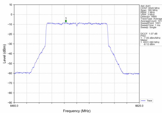
802.11ax(HEW80)_HCH_6545MHz_SU_ / Ant1_NTNV
