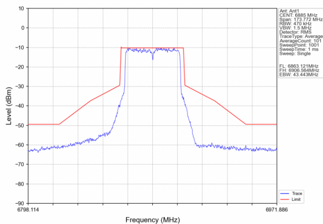
802.11ax(HEW40)_HCH_6885MHz_SU_ / Ant1_NTNV
