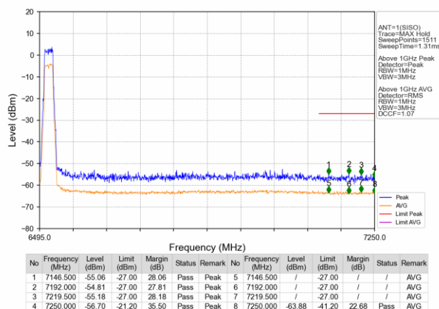
802.11ax(HEW20) HCH 6515MHz_SU / Ant1_NTNV
