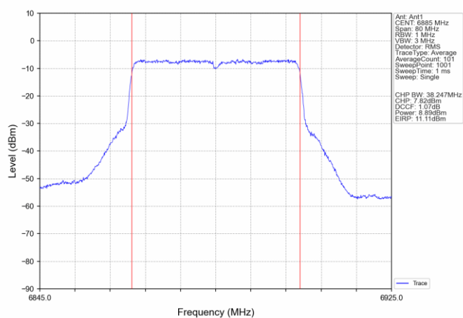
802.11ax(HEW40)_HCH_6885MHz_SU_ / Ant1_NTNV
