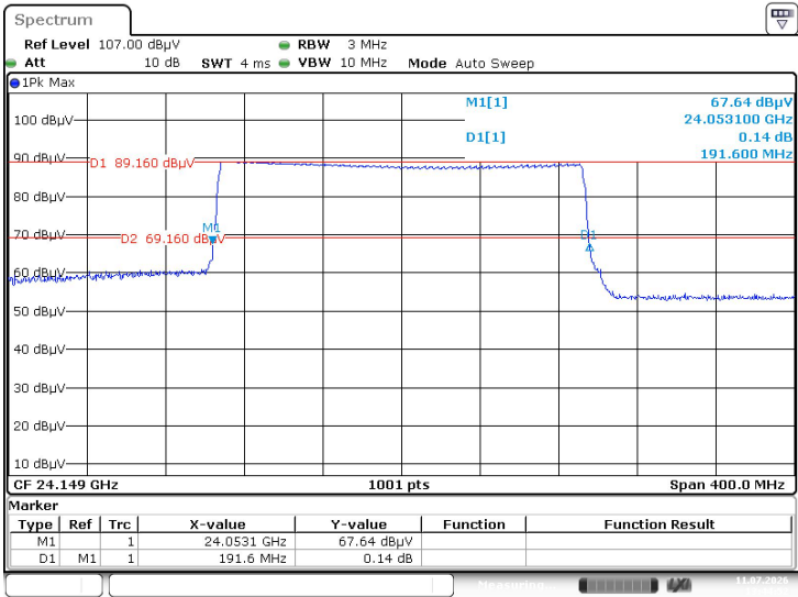
20 dB Bandwidth
