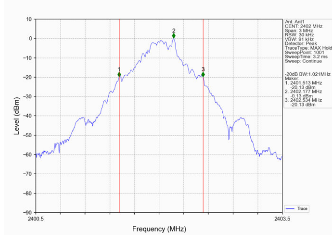
GFSK_DH5_LCH_2402MHz_Ant1_NTNV
