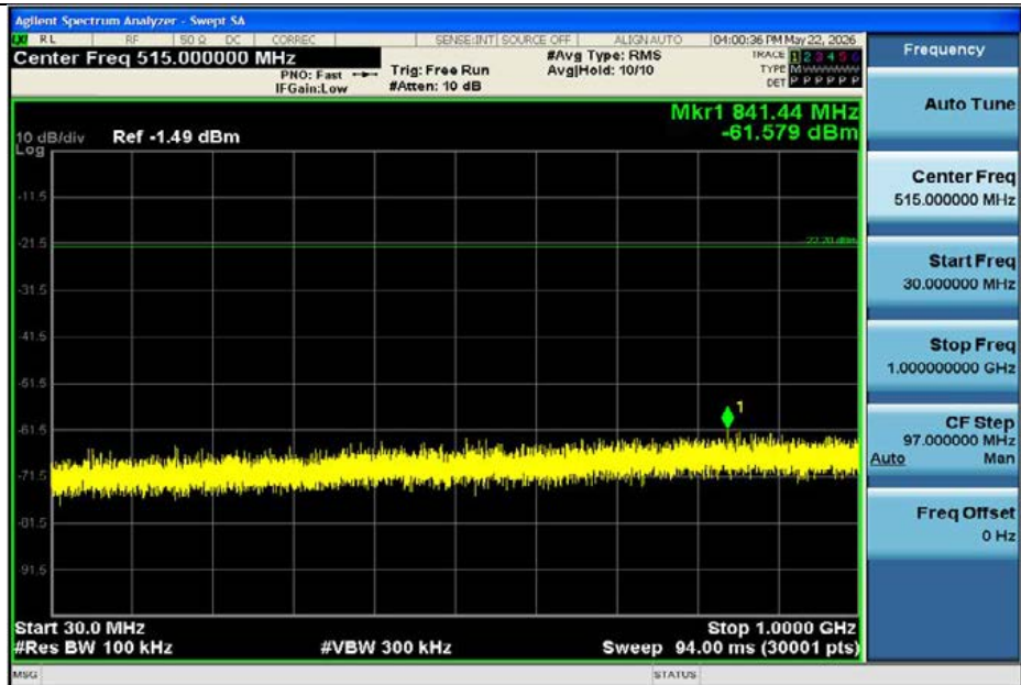
DH5-Ant1-2441-30~1000-PASS
