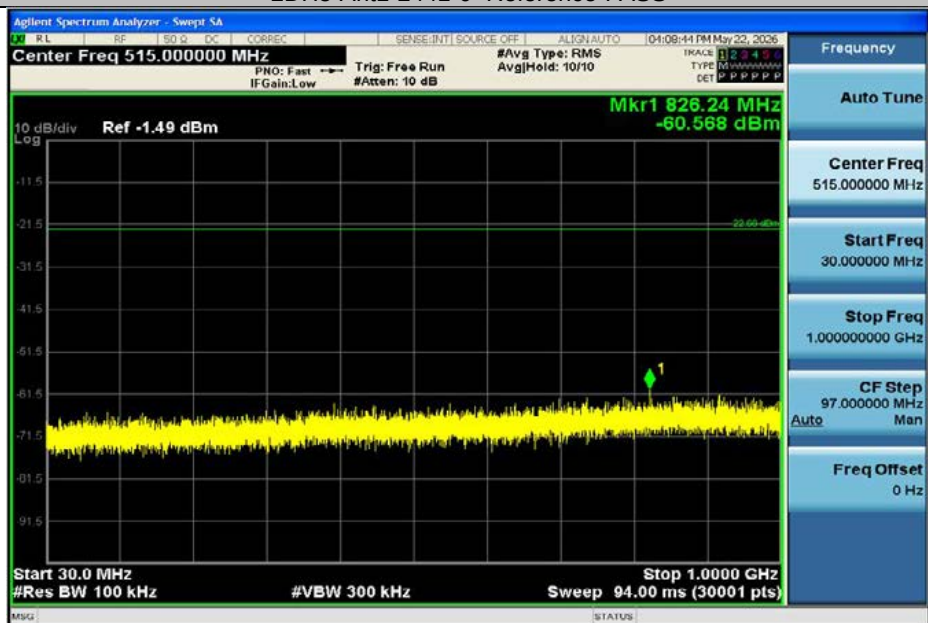
2DH5-Ant1-2441-30~1000-PASS
