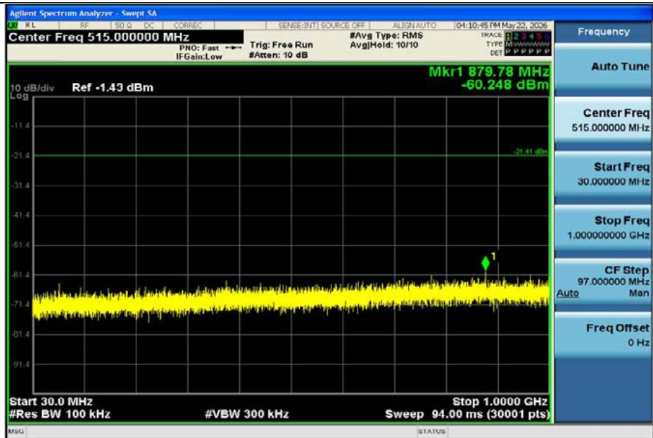
2DH5-Ant1-2480-30~1000-PASS
