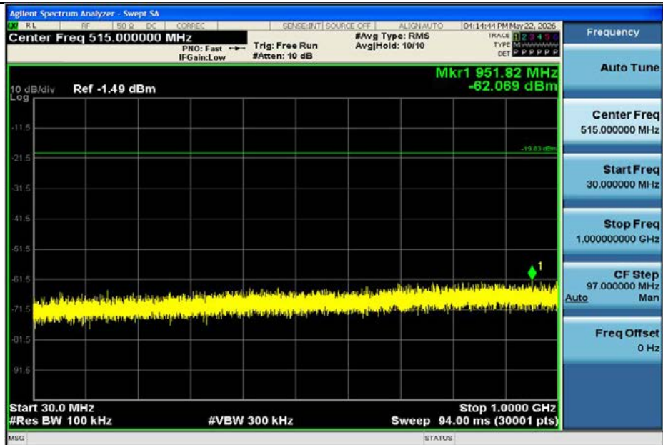
3DH5-Ant1-2441-30~1000-PASS
