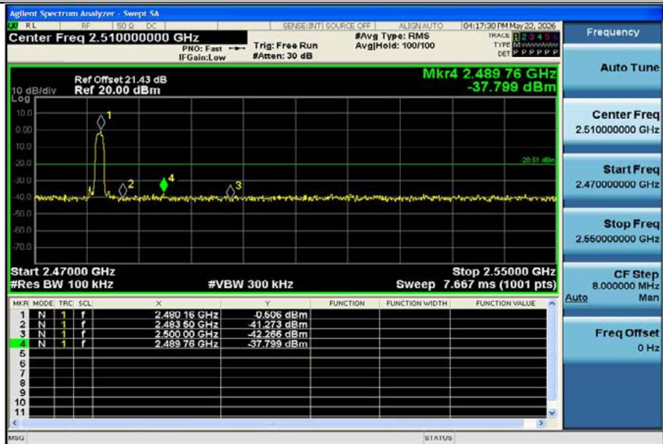
3DH5-Ant1-2480-PASS
