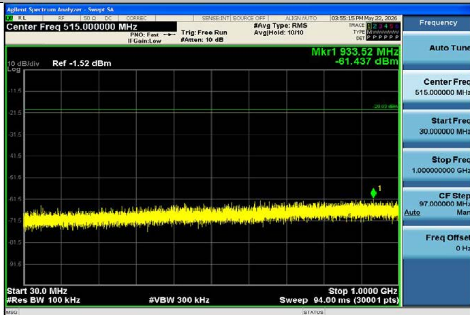
DH5-Ant1-2402-30~1000-PASS
