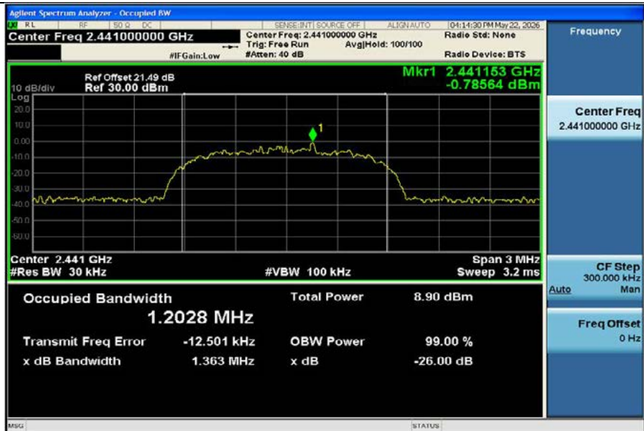
3DH5-Ant1-2441
