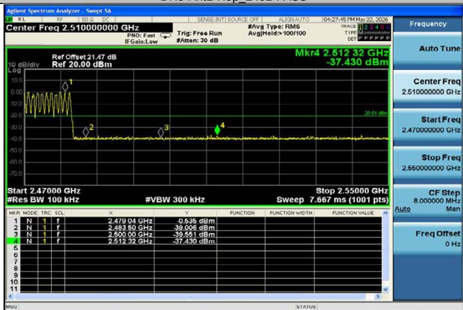
DH5-Ant1-Hop_2480-PASS
