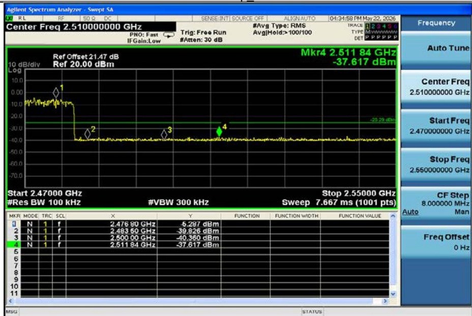
2DH5-Ant1-Hop_2480-PASS
