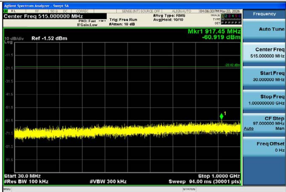
2DH5-Ant1-2402-30~1000-PASS
