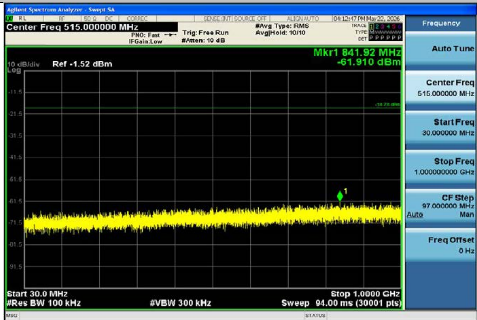
3DH5-Ant1-2402-30~1000-PASS
