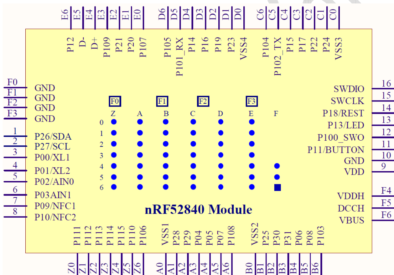
Figure 2-2 Pins assignment
