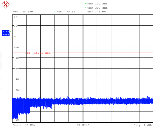
[Chart] Tx 2402MHz 1Mbps
