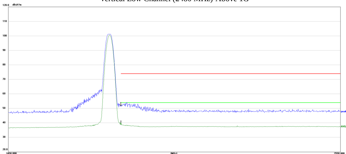
Vertical Low Channel (2480 MHz)-Above 1G
