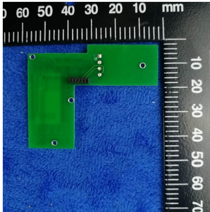
Smallboard - Rear View
