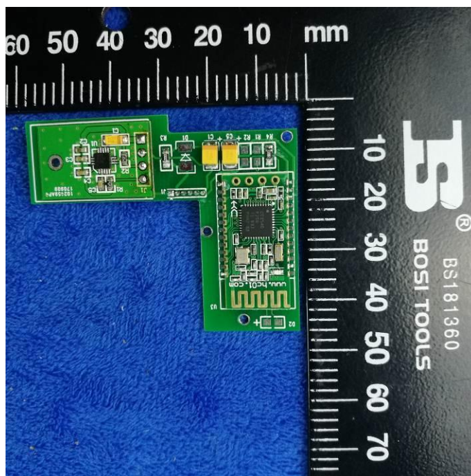
Smallboard – Front View
