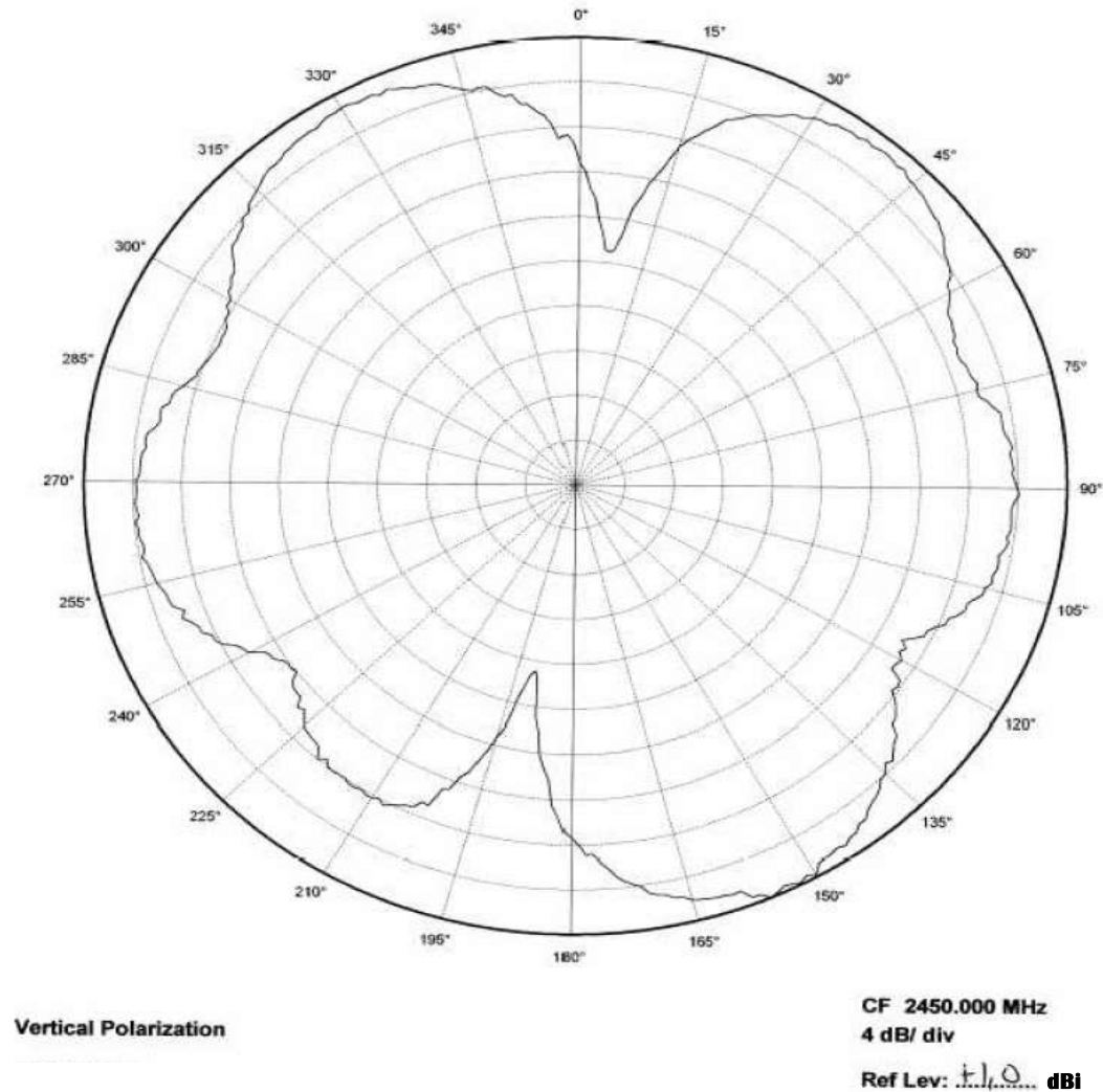
Figure 3. XY Plane–Vertical Polarization
