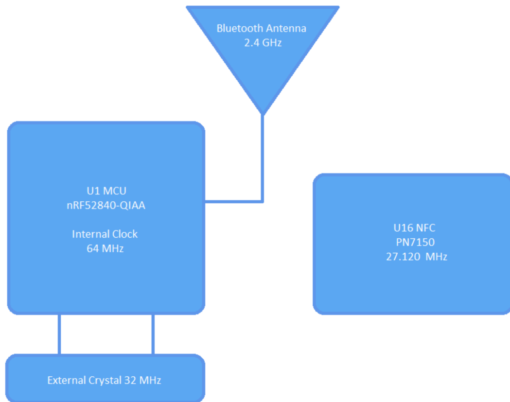
Figure 1: Block diagram and frequencies of MPS transmitter PCB
