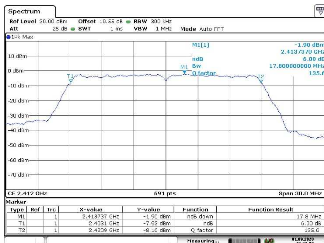
DTS Bandwidth, 2412 MHz, 802.11g, 1Mb
