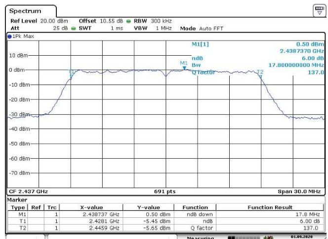
DTS Bandwidth, 2437 MHz, 802.11g, 1Mb
