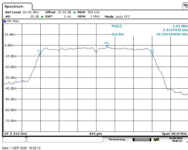
99% Occupied BW, 2412 MHz, 802.11n, HT20
