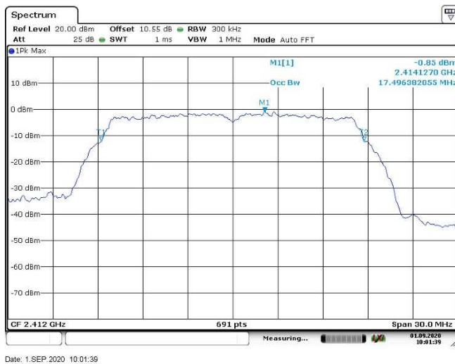
99% Occupied BW, 2412 MHz, 802.11g, 6Mb
