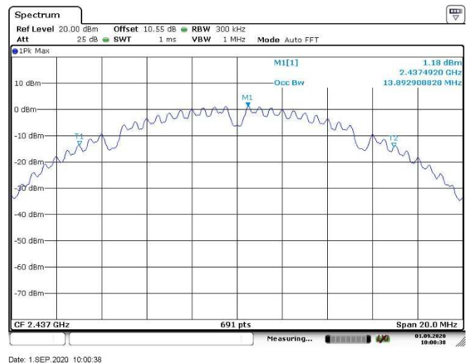
99% Occupied BW, 2437 MHz, 802.11b, 1Mb
