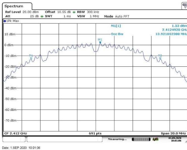
99% Occupied BW, 2412 MHz, 802.11b, 1Mb
