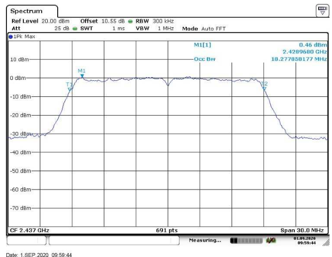
99% Occupied BW, 2437 MHz, 802.11n, HT20
