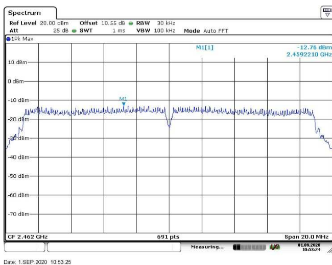
PSD, 2462 MHz, 802.11n, HT20
