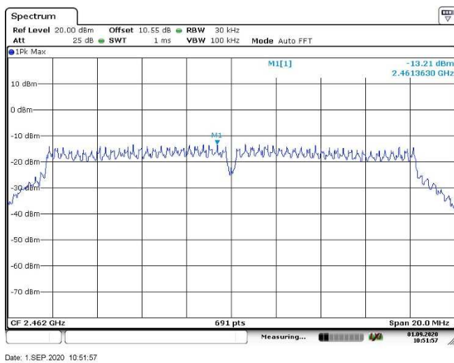
PSD, 2462 MHz, 802.11g, 6Mb
