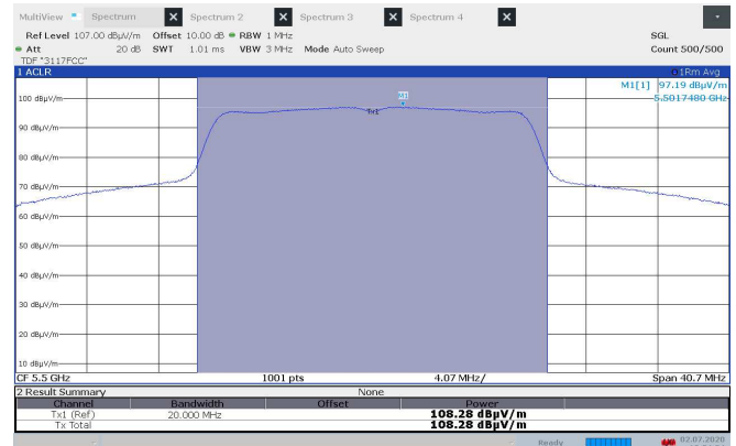
EIRP, 5500 MHz, 802.11n, HT20, Ant 1, VP, Max
