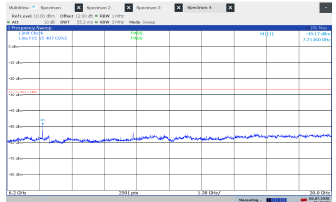
Unwanted Emissions 6.2-20 GHz, ch157, 802.11n HT20, Conducted
