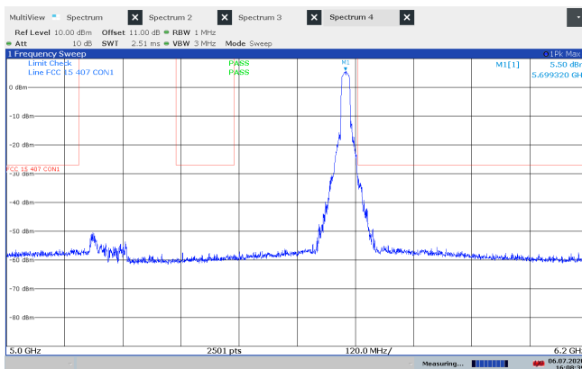
Unwanted Emissions 5000-6200 MHz, ch140, 802.11a 6Mb, Conducted
