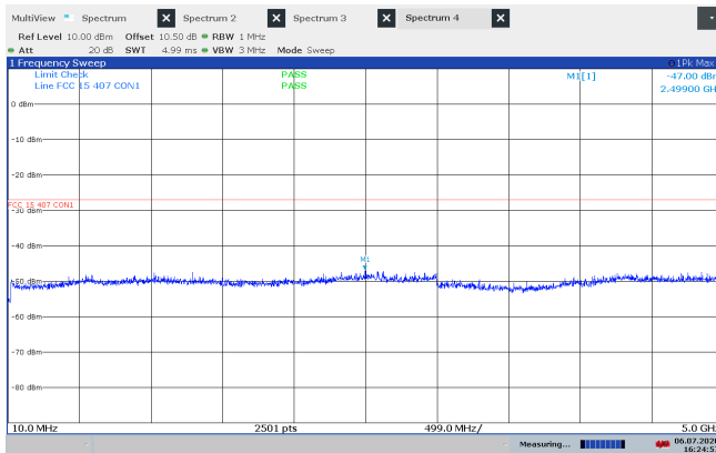
Unwanted Emissions 10-5000 MHz, ch052, 802.11a 6Mb, Conducted
