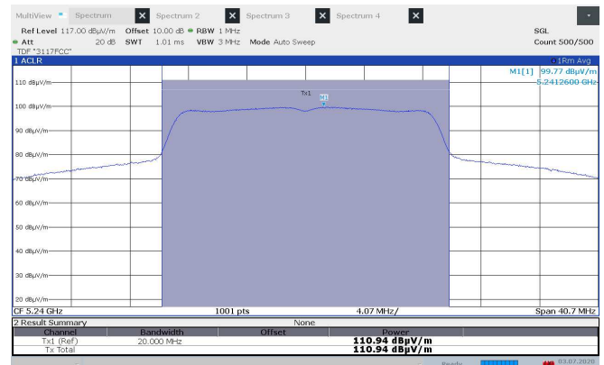
EIRP, 5240 MHz, 802.11n, HT20, Ant 2, VP, Max
