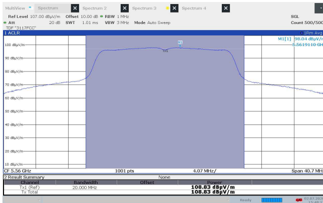
EIRP, 5560 MHz, 802.11a, 6Mb, EUT V, Ant 1, VP, Max
