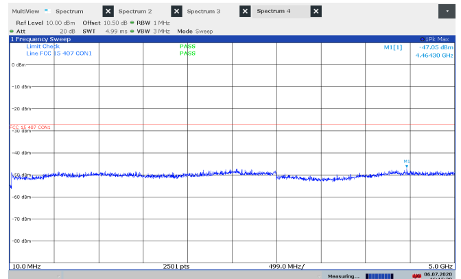
Unwanted Emissions 10-5000 MHz, ch112, 802.11n HT20, Conducted
