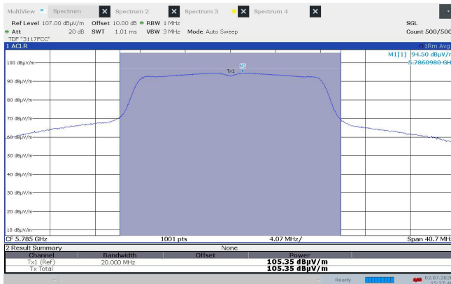
EIRP, 5785 MHz, 802.11a, 6Mb, EUT V, Ant 1, VP, Max
