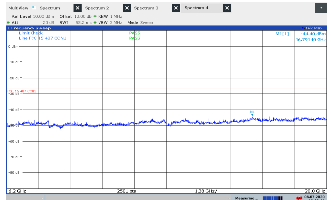
Unwanted Emissions 6.2-20 GHz, ch112, 802.11n HT20, Conducted
