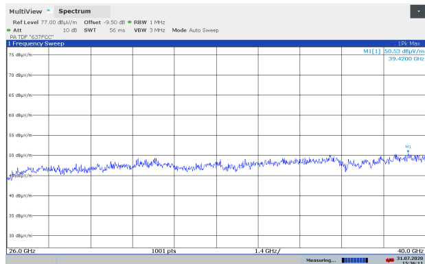
Emissions 26-40 GHz, Ch112, 802.11n HT20, Ant2, VP, @1m
