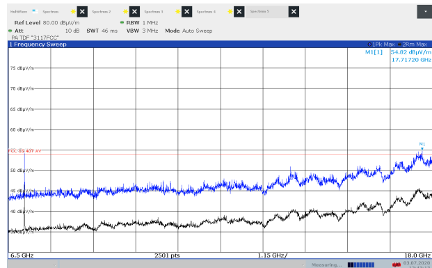
Radiated Emissions 6.5-18 GHz, Ch040, 802.11a 6M, EUT V, Ant 2, VP
