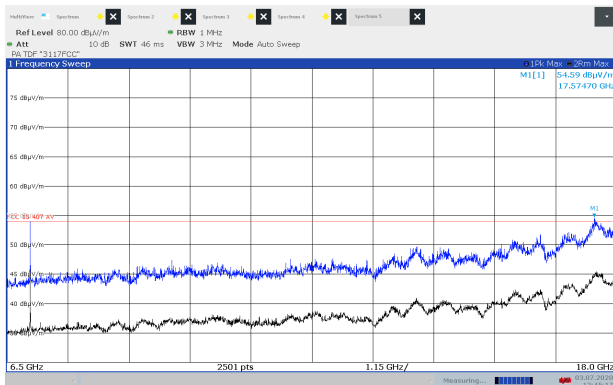
Radiated Emissions 6.5-18 GHz, Ch040, 802.11a 6M, EUT V, Ant 2, HP
