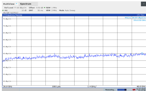
Emissions 26-40 GHz, Ch157, 802.11a 6M, Ant1, VP, @1m
