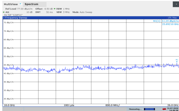
Emissions 18-26 GHz, Ch112, 802.11a 6M, Ant2, VP, @1m
