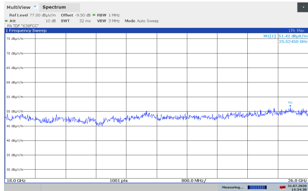
Emissions 18-26 GHz, Ch112, 802.11a 6M, Ant1, VP, @1m
