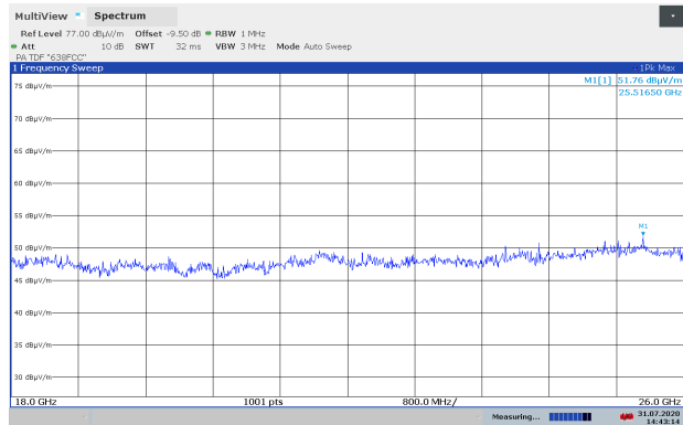
Emissions 18-26 GHz, Ch040, 802.11a 6M, Ant2, VP, @1m
