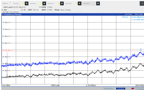
Radiated Emissions 6.5-18 GHz, Ch040, 802.11n HT20, EUT V, Ant 2, HP
