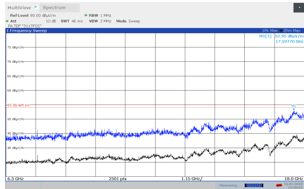
Radiated Emissions 6.5-18 GHz, Ch157, 802.11a 6M, EUT V, Ant 1, VP
