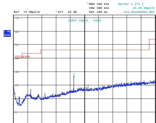
Radiated Emissions 30-1000 MHz, 802.11a 6M, EUT V, HP
