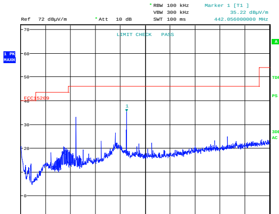
Radiated Emissions 30-1000 MHz, 802.11a 6M, EUT V, VP
