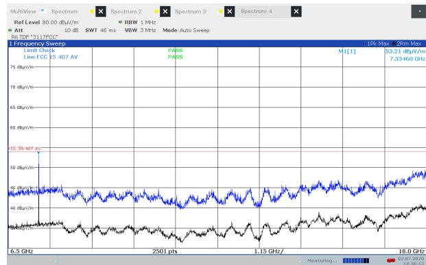
Radiated Emissions 6.5-18 GHz, Ch100, 802.11n HT20, EUT V, Ant 1, VP
