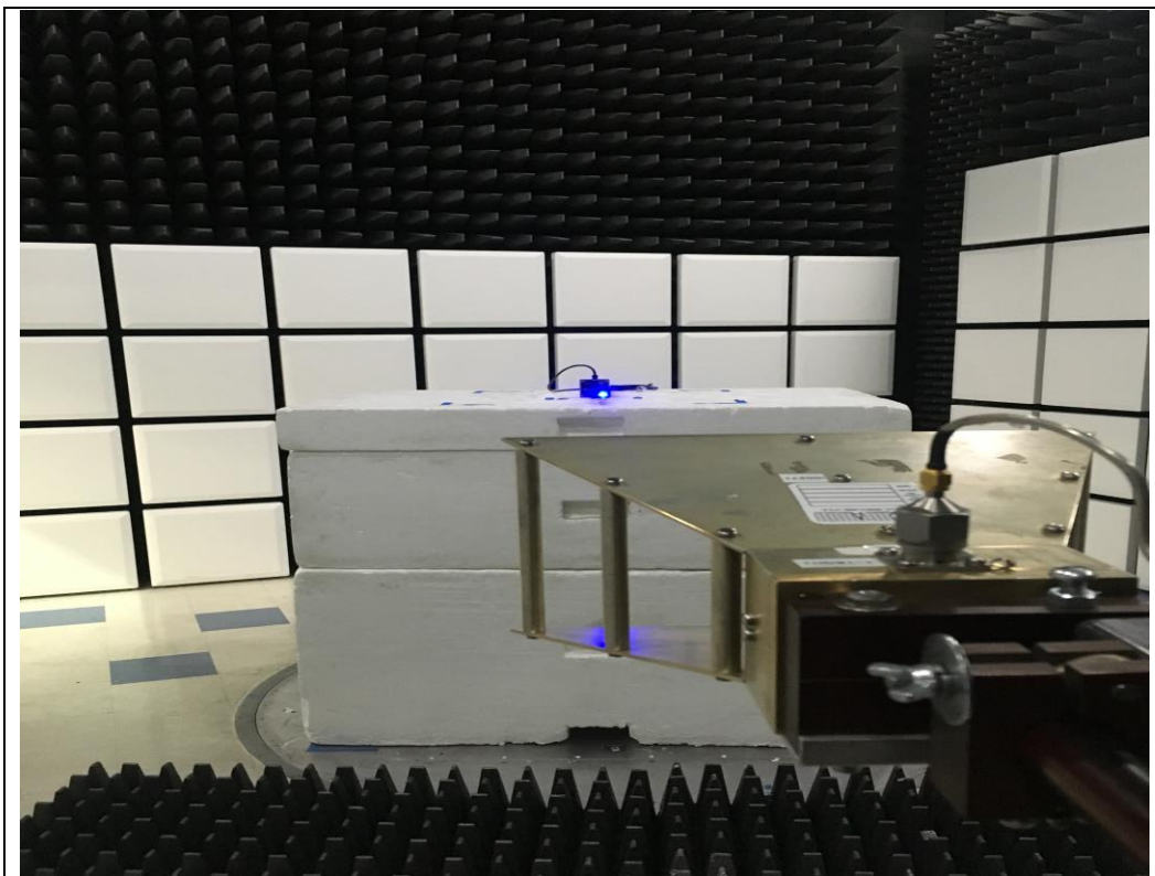
RF Radiated over 1GHz
