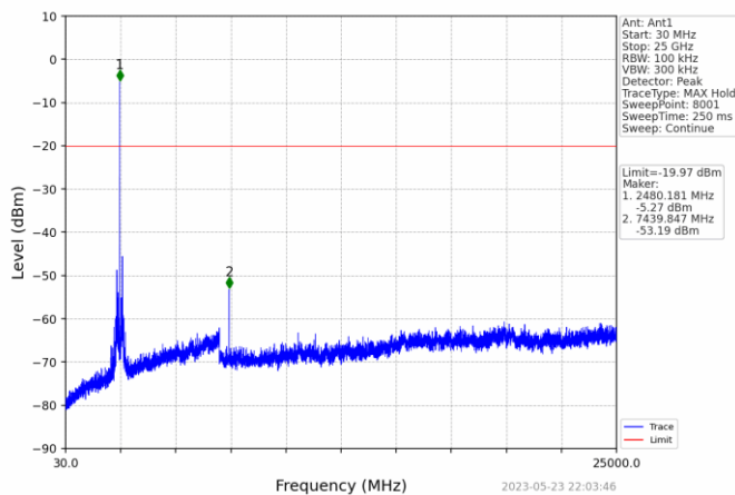
2M Full Spectrum - High Channel (2480MHz)
