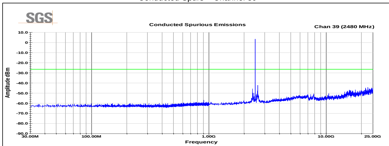
Conducted Spurs – Channel 39
