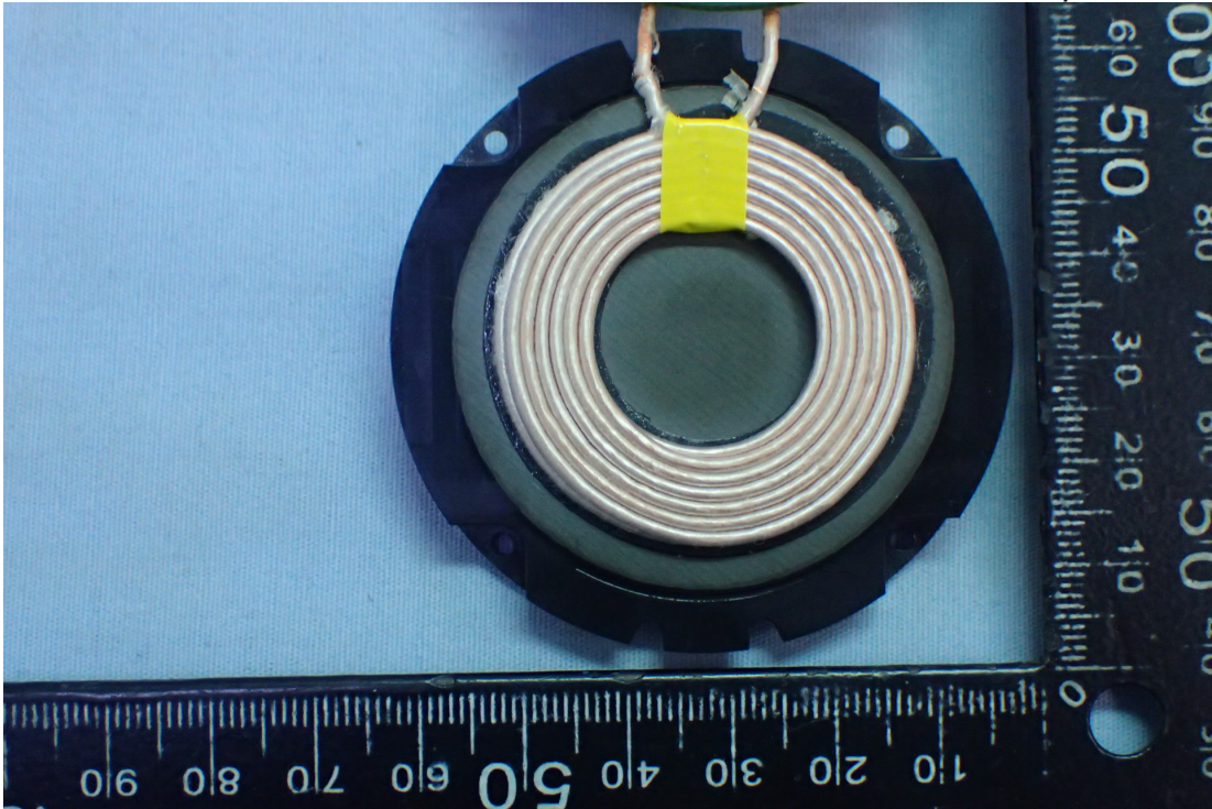
Figure 10 Loop Antenna
