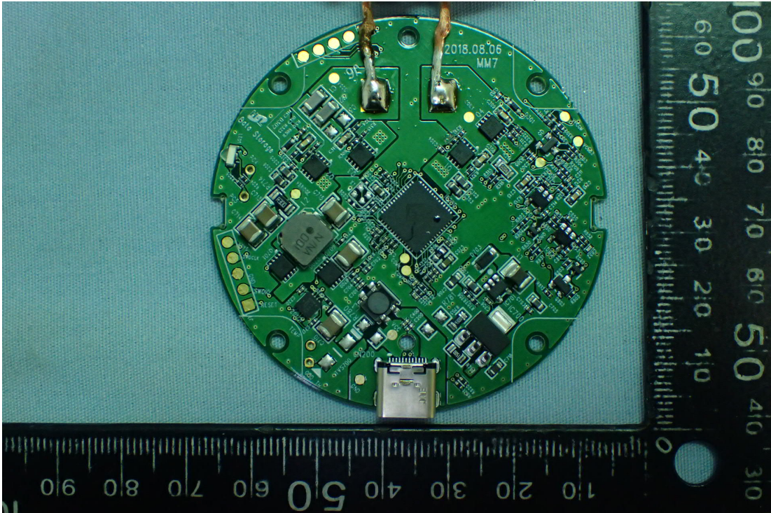
Figure 11 Internal View (Main Board, Front View)
