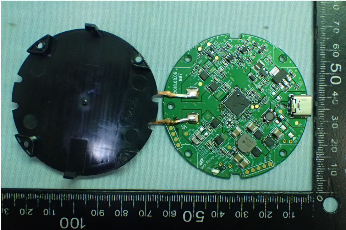
Figure 9 Internal View
